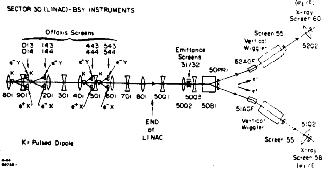
Fig. 1. Overview of the transverse beam profile and energy spread monitoring and feedback systems.
