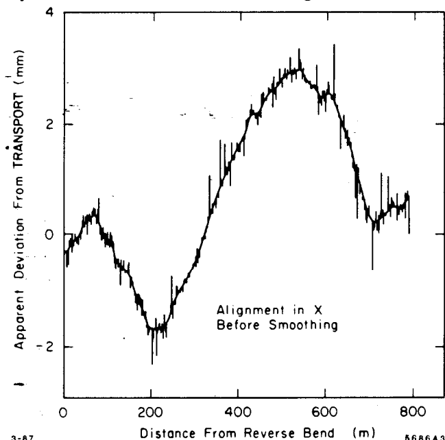
Fig. 4 Smooth curve fit with principal surface analysis
