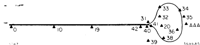
Fig. 3 Station layout for SLC Surface Survey
