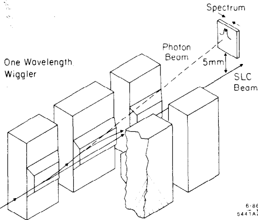
Fig. 3. Schematic of the X-ray Wiggler system used to measure \sigma_E/E in the Arcs.
