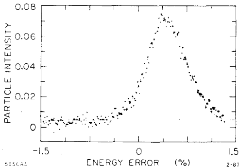
Fig. 4. Typical measurement of the energy spectrum for an individual bunch using the X-ray Wigglers (with the beam-off background distribution subtracted). The energy is measured relative to 47 GeV.
