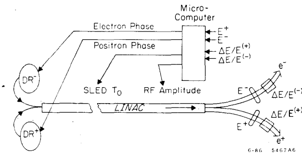
Fig. 1. Overview of the energy jitter/energy spread feedback system.
