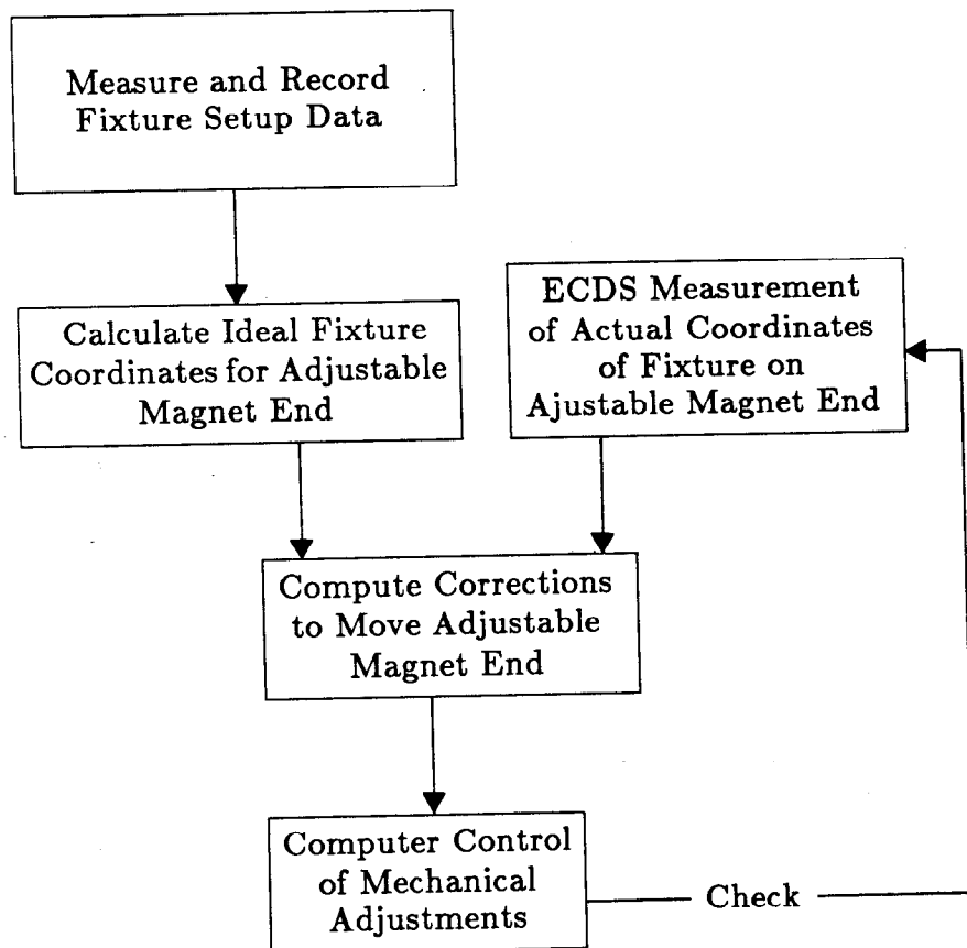
Figure 2. MAS Layout
