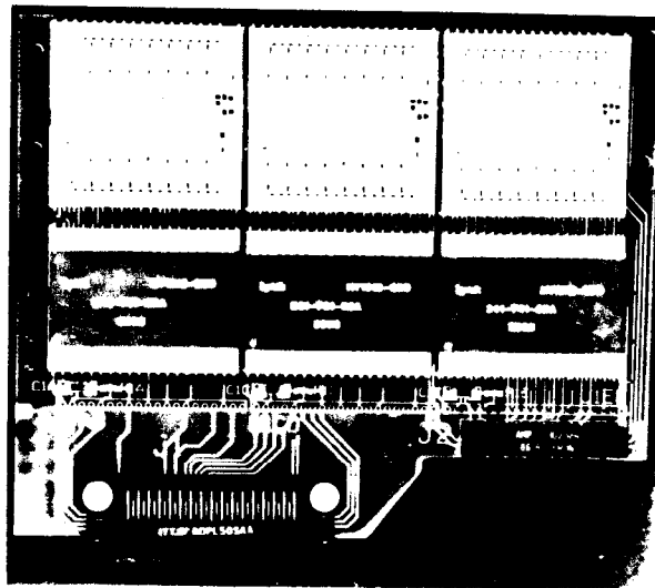
Fig. 5. Photograph of LAC 'daughter'-board serving 48 calorimeter towers.
