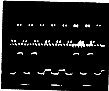
Fig. 7. Typical raw output data, repeated on an expanded time scale ( 2 \mu\text{s}/\text{div} ) in the lower half of the figure. Vertical scale is 1 \text{ V}/\text{div} . The read-out sequence is: Two signal channels at gain 1, each in the order signal and baseline. This is followed by the same channels at gain 8. The pattern is then repeated for all channels.
