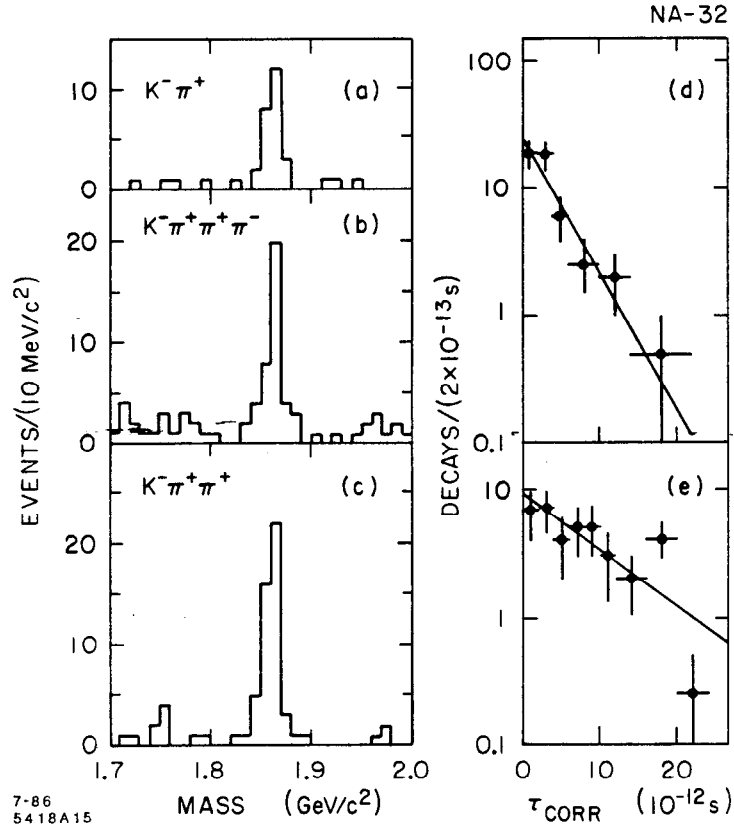
Fig. 2. NA-32: Effective mass and corrected decay time distributions for the selected D mesons.
