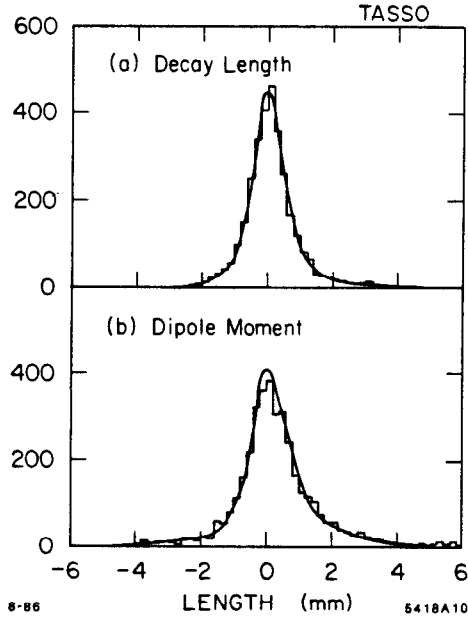
Fig. 9. TASSO: Distribution of a) the "decay length" and b) the "dipole moment". The solid curve shows the result of a Monte Carlo simulation with the B lifetime and fragmentation adjusted to fit the data.
