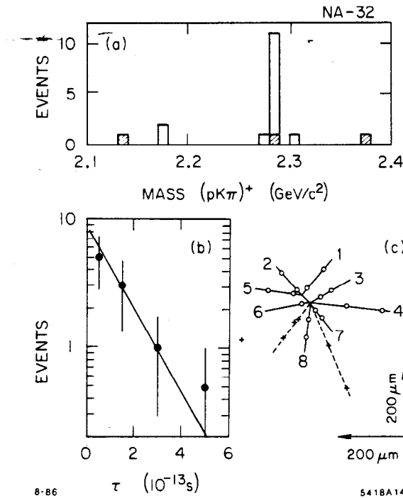
Fig. 3. NA-32: Measurement of the \Lambda_c lifetime, a) effective mass, b) decay time distribution and c) a display of a single event detected in the CCDs (tracks 1,2,5 result from a \Lambda_c decay).
