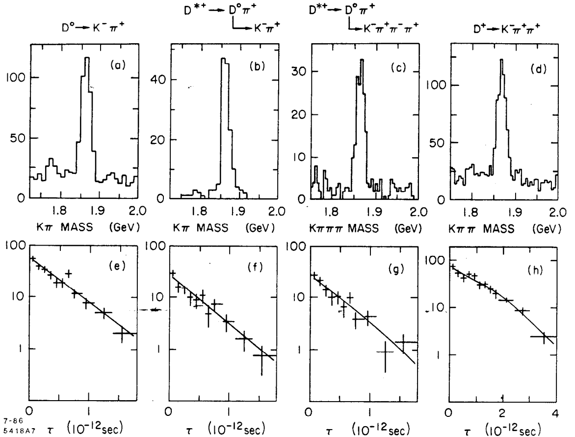
Fig. 4. E-691: Effective mass and decay time distributions for selected D decays.
