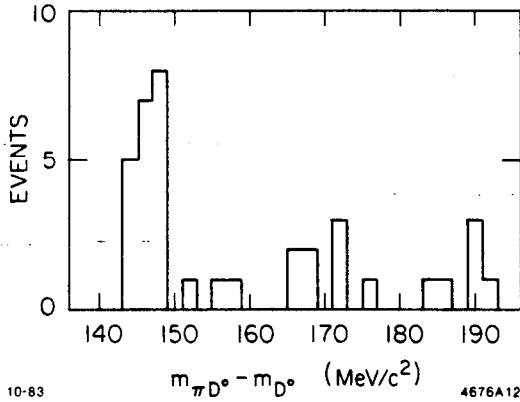
Fig. 1. Mass difference m_{K^{\mp}\pi^{\pm}\pi^{\pm}} - m_{K^{\mp}\pi^{\pm}} for K^{\mp}\pi^{\pm} combinations near the D^0 mass and E_{K\pi\pi}/E_{beam} > .6 .
