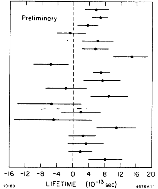
Fig. 2. Measured D^0 Lifetimes.
