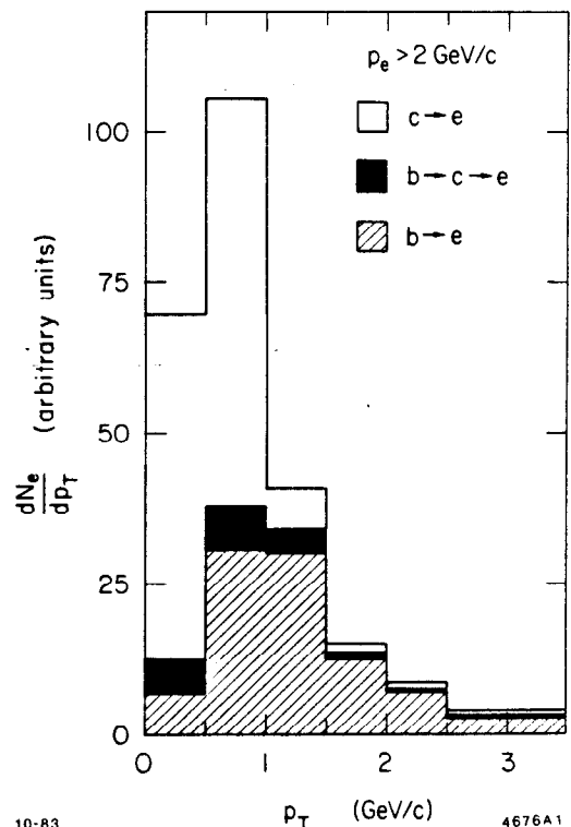
Fig. 3. Transverse momentum spectrum of prompt electrons produced in e^+e^- annihilations at 29 GeV. The highest bin includes all leptons with transverse momenta above 3 GeV/c.
