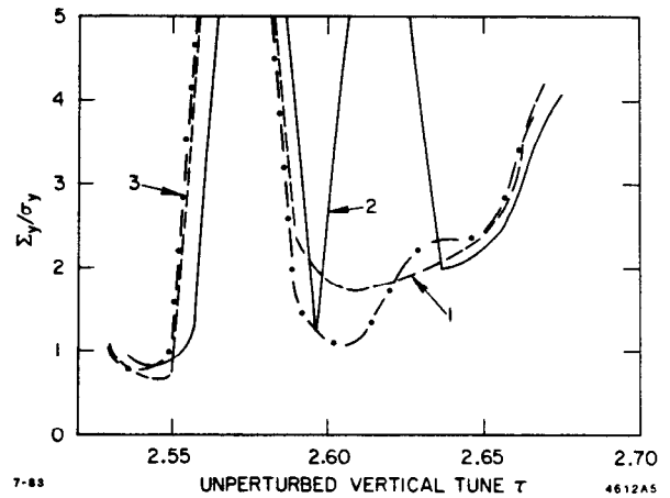
Fig. 5. Beam blowup versus unperturbed vertical tune (per one superperiod). The calculations are done using the case B formula for strong beam current 8 mA. The same machine parameters are assumed as for the curve 1 on Fig. 4 but the unperturbed horizontal tune. Curves 1, 2, and 3 correspond to values \nu = 2.62, 2.64 (nominal value for SPEAR), and 2.66. The nominal vertical tune for SPEAR is 2.59.
