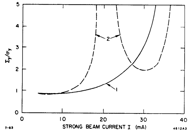
Fig. 3. Strong dependence on the assumed asymmetry values is illustrated in this figure. Curve 1 is the same as curve 2 on Fig. 1. Curve 2 is calculated with \Delta\nu and \Delta\tau twice as big (the rest of the parameters are the same).
