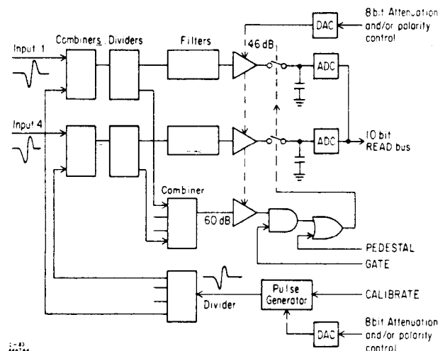
Fig. 4. Block diagram of the position monitor electronics.
