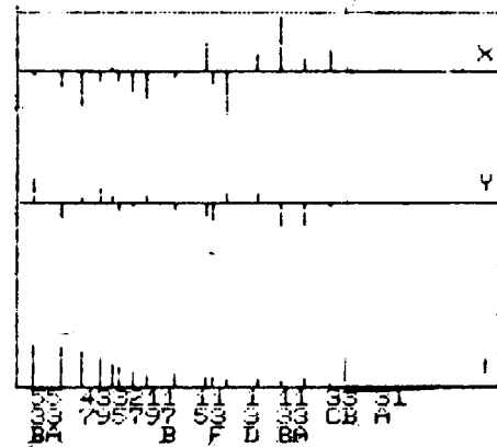
Fig. 8. Beam position (mm) and transmission (arbitrary units) along the Linac to Damping Ring transfer line at turn on.
