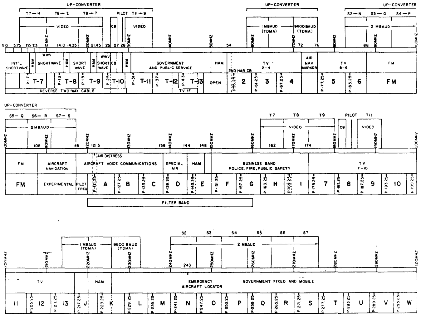
SLC BROADBAND CABLE SPECTRUM
