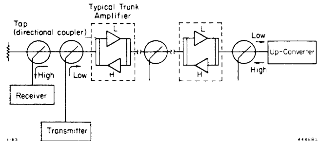
Fig. 1. Basic signal flow on the cable.
