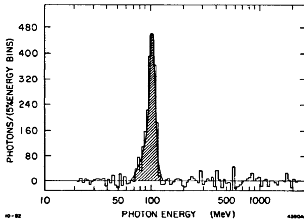
Fig. 12: The CUSB detector's photon energy resolution curve at about E_\gamma = 100 MeV, as determined from Monte Carlo calculations.
