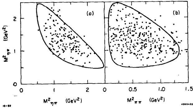
Fig. 22: The Dalitz plots for J/\psi + \gamma\eta\pi^+\pi^- events with 1600 < M_{\eta\pi\pi} < 1850 MeV. The boundaries are calculated for M_{\eta\pi\pi} = 1710 MeV. Note that part (b) has two entries per event.
