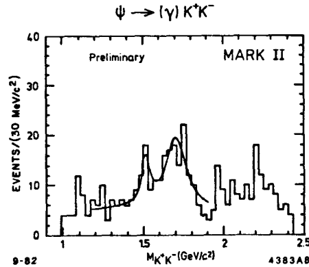
Fig. 18: A preliminary M_{K^+K^-} distribution from J/\psi \rightarrow (\gamma) K^+K^- (Mark II Collaboration). The solid line is the fit described in the text (cf Eq. (45)). Signals at the f' and \theta are obtained.
