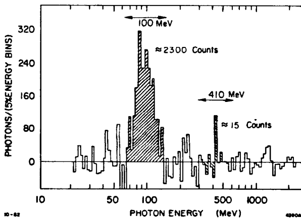
Fig. 6: The photon signal obtained from the data shown in Fig. 5 by subtracting the smooth curve from the measured data. An impressive bump is seen at about 100 MeV, with no other structure evident. A twelve bin slice about 410 MeV yields about 15 counts.
