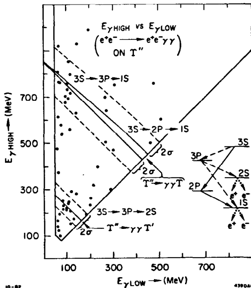
Fig. 7: The lower photon energy versus the higher photon energy from T'' \rightarrow \gamma\gamma e^+e^- events. The 2\sigma resolution bands are shown. The data is from CUSB. [16]
