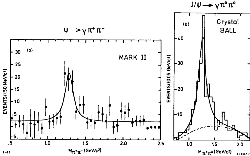
Fig. 17: a) M_{\pi\pi} mass distribution from J/\psi \rightarrow \gamma\pi^+\pi^- (the Mark II Collaboration) the fit represents fit to f(1270) plus background. b) M_{\pi\pi} mass distribution from J/\psi \rightarrow \gamma\pi^0\pi^0 (Crystal Ball Collaboration). The solid curve represents a fit to f(1270) plus background. The dashed curve represents the background estimate.
