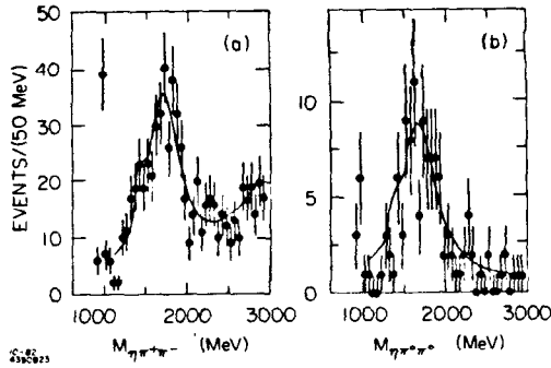
Fig. 21: a) \eta\pi^+\pi^- and b) \eta\pi^0\pi^0 mass spectra for J/\psi + \gamma\eta\pi\pi events. The solid curve is a two resonance fit, one resonance fixed at the \iota mass and width and having variable amplitude, the other having all parameters variable. The mass, width and amplitude of the broad structure seen in the figures is essentially given by Eqs. (52) and (53). The \iota upper limit obtained from the fit is given in Table 5.
