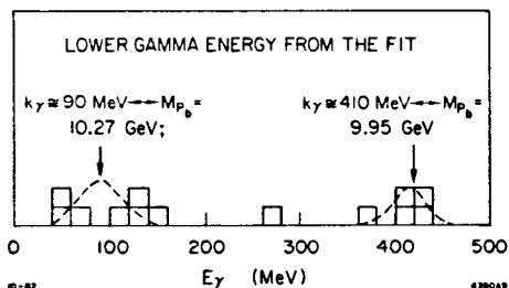
Fig. 10: The lower photon energy distribution obtained from the fits discussed in the text and Fig. 9. The CLEO Collaboration[16] claims two peaks indicating the observation of two P_b states, one at k_\gamma \approx 90 MeV, the other at k_\gamma \approx 410 MeV.
