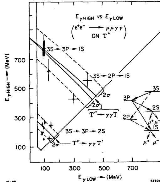
Fig. 8: The lower photon energy versus the higher photon energy from T'' \rightarrow \gamma\gamma \mu^+\mu^- events. The 2\sigma resolution bands are shown. The data is from CUSB. [16]
