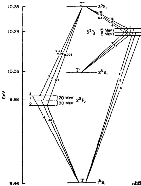
Fig. 4: The ^3S_1 , ^3P_J spectrum which many theories expect for the b\bar{b} bound system. The energy of the bound states is shown in GeV on the ordinate scale. Typical expectations for the ^3P_J fine structure is also shown. Two examples of transition rates are shown for n^3S_1 + \gamma n^3P_J transitions. The top set of numbers is from Ref. [2], the bottom set from Ref. [18]. Only the results from Ref. [18] are shown for the other transitions. See also Ref. [1].
