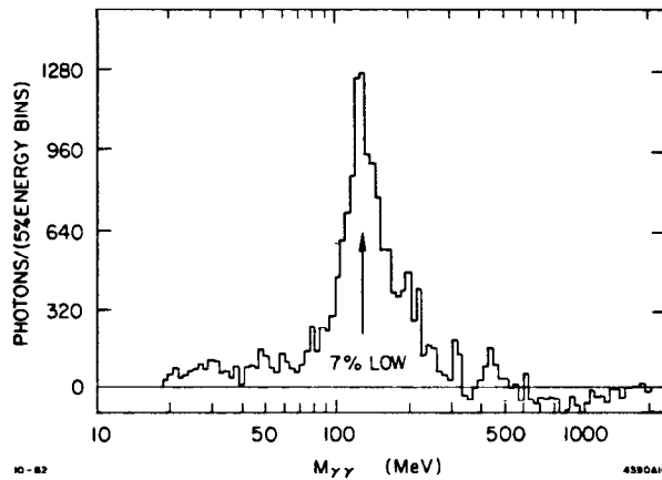
Fig. 11: M_{\gamma\gamma} distribution from CUSB.[16] The \pi^0 mass is about 7% low. These data are used to calibrate the photon energy scale as discussed in the text.
