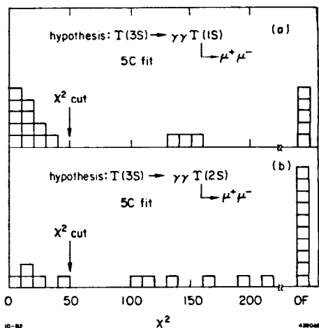
Fig. 9: The \chi^2 distribution from 5-c fits to events with hypothesis, a) T(3S) \rightarrow \gamma\gamma T(1S) + \gamma\gamma\mu^+\mu^- , and b) T(3S) \rightarrow \gamma\gamma T(2S) + \gamma\gamma\mu^+\mu^- . The data are from the CLEO Collaboration.[16] Events are accepted with \chi^2 \leq 50 .
