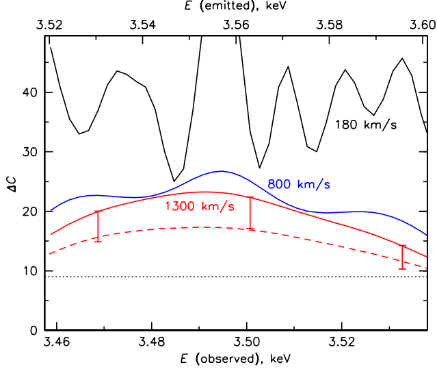
Fig. 2.— Difference of C statistic between a model with a line with the best-fit XMM MOS flux ( 9 \times 10^{-6} phot s^{-1} cm^{-2} ) and the best-fit SXS flux (shown in Fig. 3; flux is allowed to take negative values) as a function of line energy within the B14 most restrictive confidence interval for the line. Curves for different line widths are shown (black: 180 km\ s^{-1} , blue: 800 km\ s^{-1} , red: 1300 km\ s^{-1} ). For the 1300 km\ s^{-1} case, we also show \Delta C between models with the XMM MOS line flux and zero line flux (red dashed line). Error bars illustrate a systematic uncertainty of the SXT effective area described in §3.1; its effect is most significant for the broad line and we do not show other cases for clarity. Dotted line is at \Delta C = 9 , which corresponds to 3\sigma exclusion for Gaussian errors.
