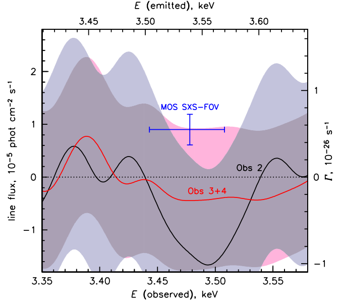
FIG. 5.— The best-fit flux (curves) and \pm 3\sigma limits (shaded bands) for a 1300 km s -1 broadened line (similar to the red line and pink band in Fig. 3), derived separately for the early subset (“Obs 2”, black and gray) and later subset (“Obs 3+4”, red and pink). The axes and the blue cross are the same as in Fig. 3. The “dip” around 3.5 keV is present in the early subset and not in the late one, but the results are statistically consistent.
