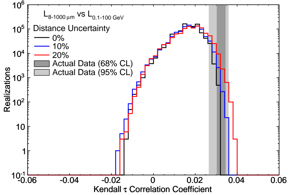
FIG. 5.— Graphical representation of the method adopted to estimate significances of multiwavelength correlations using the Kendall \tau statistic. Total IR luminosity ( 8\text{--}1000\ \mu\text{m} ) and gamma-ray luminosity ( 0.1\text{--}100\ \text{GeV} ) are compared using the full sample of 69 galaxies in this example. Null hypothesis distributions of correlation coefficients assuming independence between wavebands are shown for 3 levels of uncertainty in distance measurements (1 standard deviation of the scatter). The null hypothesis distributions are generated from 10^6 permutations of gamma-ray luminosities among the galaxies, requiring that the resultant gamma-ray fluxes could have been measureable given the flux sensitivity threshold of the LAT. The correlation coefficient of the actual data is represented as a probability density to account for uncertainty in measured gamma-ray fluxes. The gray bands indicate the inner 68% and 95% of the probability density for the actual data. The correlation significance is estimated by computing the fraction of null hypothesis realizations with correlation coefficient larger than that obtained for the actual data (i.e. the P -value). See Section 4.3 and Appendix A for details.
