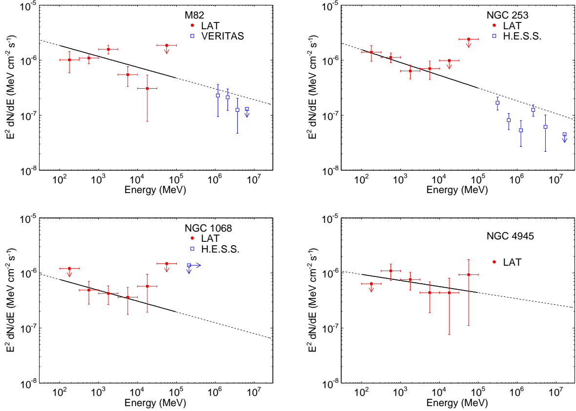
FIG. 2.— Spectral energy distributions for four starburst galaxies significantly detected in high energy gamma rays. 95% confidence upper limits are indicated in energy bins with detection significance TS < 1 . The best-fit power law spectral model is shown for each galaxy in the energy range used for the maximum likelihood analysis (0.1–100 GeV; solid) and in extrapolation to neighboring wavebands (dashed). Flux measurements produced by imaging air-Cherenkov telescopes are included for M82 (VERITAS, Acciari et al. 2009) and NGC 253 (H.E.S.S., Ohm et al. 2011), and flux upper limits above 210 GeV are shown for NGC 1068 (H.E.S.S., Aharonian et al. 2005). The uncertainties depicted for LAT flux measurements represent combined statistical and systematic uncertainties.
