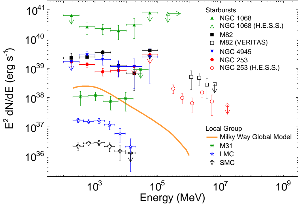
FIG. 6.— Gamma-ray luminosity spectra of star-forming galaxies detected by the LAT and imaging air-Cherenkov telescopes.
