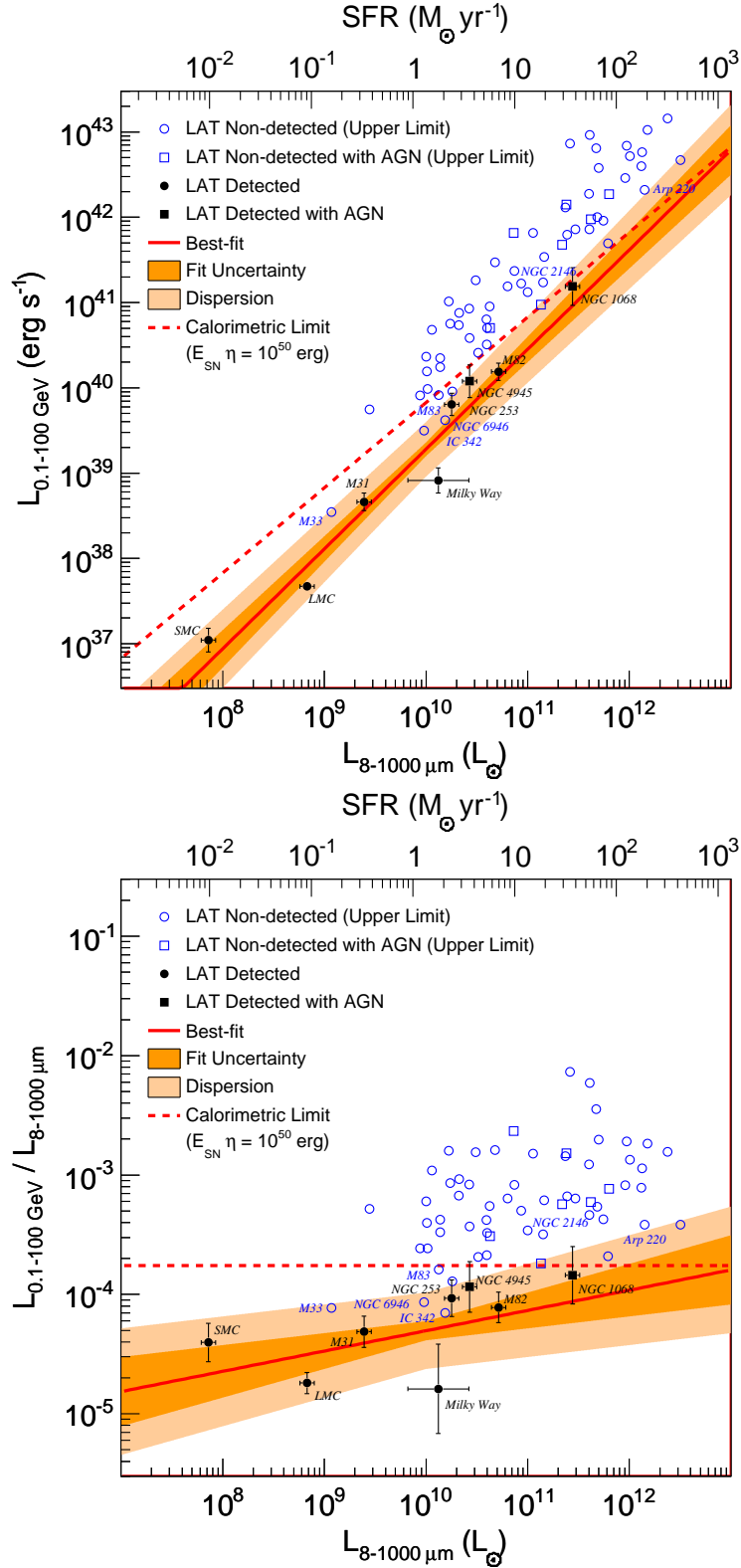
FIG. 4.— As Figure 3, but showing gamma-ray luminosity (0.1–100 GeV) versus total IR luminosity (8–1000 \mu\text{m} ). IR luminosity uncertainties for the non-detected galaxies are omitted for clarity, but are typically \sim 0.06 dex. The upper abscissa indicates SFR estimated from the IR luminosity according to equation 1 (Kennicutt 1998b).
