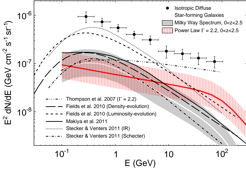
FIG. 7.— Estimated contribution of unresolved star-forming galaxies (both quiescent and starburst) to the isotropic diffuse gamma-ray emission measured by the Fermi LAT (black points, Abdo et al. 2010h). The shaded regions indicate combined statistical and systematic uncertainties in the contributions of the respective populations. Two different spectral models are used to estimate the GeV gamma-ray emission from star-forming galaxies: a power law with photon index 2.2, and a spectral shape based on a numerical model of the global gamma-ray emission of the Milky Way (Strong et al. 2010). These two spectral models should be viewed as bracketing the expected contribution since multiple star-forming galaxy types contribute, e.g. dwarfs, quiescent spirals, and starbursts. We consider only the contribution of star-forming galaxies in the redshift range 0 < z < 2.5 . The gamma-ray opacity of the Universe is treated using the extragalactic background light model of Franceschini et al. (2008). Several previous estimates for the intensity of unresolved star-forming galaxies are shown for comparison. Thompson et al. (2007) treated starburst galaxies as calorimeters of CR nuclei. The normalization of the plotted curve depends on the assumed acceleration efficiency of SNRs (0.03 in this case). The estimates of Fields et al. (2010) and by Makiya et al. (2011) incorporate results from the first year of LAT observations. Fields et al. (2010) considered the extreme cases of either pure luminosity evolution and pure density evolution of star-forming galaxies. Two recent predictions from Stecker & Venter (2011) are plotted: one assuming a scaling relation between IR-luminosity and gamma-ray luminosity, and one using a redshift-evolving Schechter model to relate galaxy gas mass to stellar mass.
