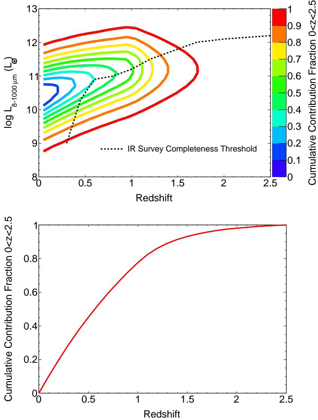
FIG. 8.— Relative contribution of star-forming galaxies to the isotropic diffuse gamma-ray background according to their redshift and total IR luminosity (8–1000 \mu\text{m} ) normalized to the total contribution in the redshift range 0 < z < 2.5 . Top Panel: Solid contours indicate regions of phase space which contribute an increasing fraction of the total energy intensity ( \text{GeV cm}^{-2} \text{s}^{-1} \text{sr}^{-1} ) from all star-forming galaxies with redshifts 0 < z < 2.5 and 10^8 L_{\odot} < L_{8-1000 \mu\text{m}} < 10^{13} L_{\odot} . Contour levels are placed at 10% intervals. The largest contribution comes from low-redshift Milky Way analogues ( L_{8-1000 \mu\text{m}} \sim 10^{10} L_{\odot} ) and starburst galaxies comparable to M82, NGC 253, and NGC 4945. The black dashed curve indicates the IR luminosity above which the survey used to generate the adopted IR luminosity function is believed to be complete (Rodighiero et al. 2010). Bottom Panel: Cumulative contribution versus redshift. As above, only the redshift range 0 < z < 2.5 is considered.
