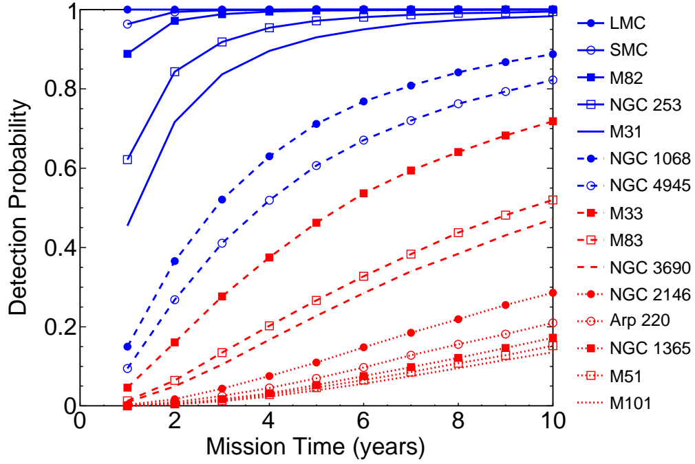
FIG. 10.— LAT detection probabilities for individual galaxies using the scaling relation found in Section 4.3. Galaxies already detected by the LAT are shown by blue curves, while other galaxies are drawn with red curves.
