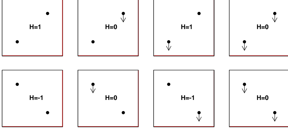
FIG. 12.— Graphical representation of the generalized Kendall \tau rank correlation test. The \tau correlation statistic is proportional to the sum of H -values obtained for each pair of points in the dataset. See Appendix A for a complete description of the method.
