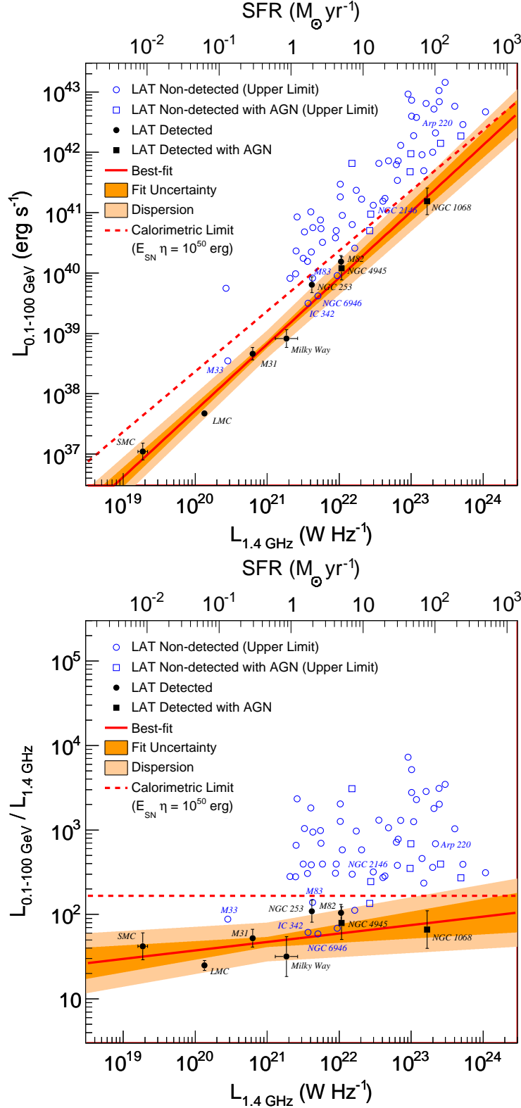
FIG. 3.— Top Panel: Gamma-ray luminosity (0.1–100 GeV) versus RC luminosity at 1.4 GHz. Galaxies significantly detected by the LAT are indicated with filled symbols whereas galaxies with gamma-ray flux upper limits (95% confidence level) are marked with open symbols. Galaxies hosting Swift -BAT AGN are shown with square markers. RC luminosity uncertainties for the non-detected galaxies are omitted for clarity, but are typically less than 5% at a fixed distance. The upper abscissa indicates SFR estimated from the RC luminosity according to equation 2 (Yun et al. 2001). The best-fit power law relation obtained using the EM algorithm is shown by the red solid line along with the fit uncertainty (darker shaded region), and intrinsic dispersion around the fitted relation (lighter shaded region). The dashed red line represents the expected gamma-ray luminosity in the calorimetric limit assuming an average CR luminosity per supernova of E_{\text{SN}} \eta = 10^{50} \text{ erg} (see Section 5.1). Bottom Panel: Ratio of gamma-ray luminosity (0.1–100 GeV) to RC luminosity at 1.4 GHz.
