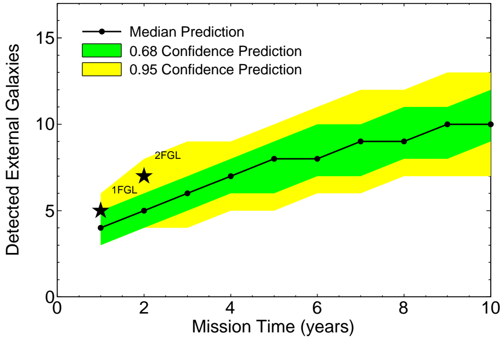
FIG. 11.— Total number of star-forming galaxies anticipated to be detected during a 10-year Fermi mission. The actual numbers of external galaxies reported in the 1FGL (Abdo et al. 2010c) and 2FGL (Nolan et al. 2012) catalogs are marked with star symbols.
