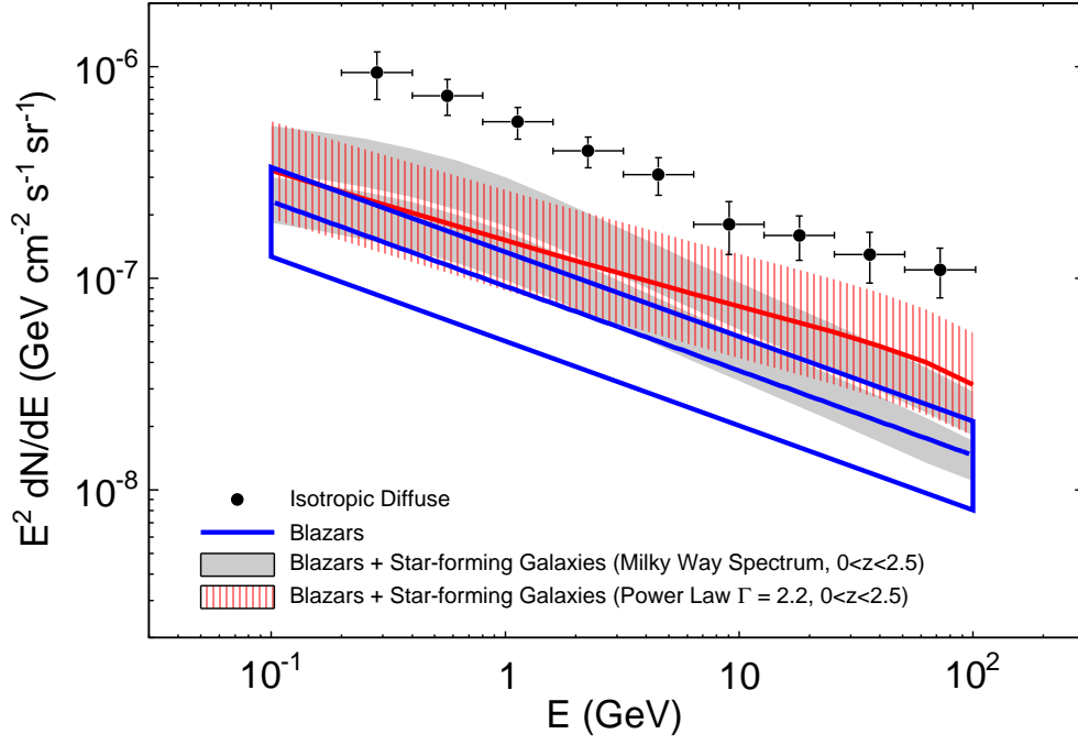
FIG. 9.— As Figure 7, but showing the summed contributions of blazars and star-forming galaxies (this work) to the isotropic diffuse gamma-ray background. Two different assumed spectral models for the star-forming galaxies are shown. The estimated contribution of blazars is derived from the distribution of observed fluxes for high Galactic latitude sources observed by the LAT, which are believed to be dominated by FSRQs and BL Lac objects (Abdo et al. 2010i).
