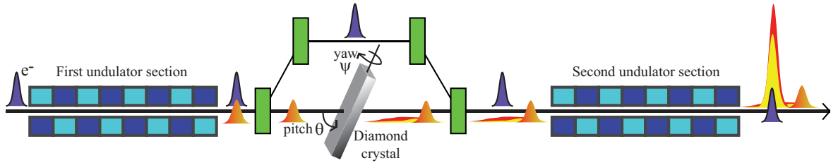
FIG. 1. Single-crystal self-seeding scheme at LCLS. In the first undulator section a self-amplified spontaneous emission (SASE) photon pulse is generated. This photon pulse diffracts from a diamond crystal. The diffracted bandwidth is at least an order of magnitude smaller than the SASE bandwidth. The diffracted beam exits at some angle to the incident beam, and is discarded. The undiffracted, transmitted pulse consists of a wide-bandwidth short pulse followed by a relatively weak narrow-bandwidth tail. The electron pulse is delayed by the magnetic chicane so that it overlaps spatially with the narrow-bandwidth tail of the X-ray pulse in the second undulator section. The narrow-bandwidth tail, with long temporal coherence length, seeds FEL amplification in the second undulator section, generating a narrow-band intense X-ray output.
