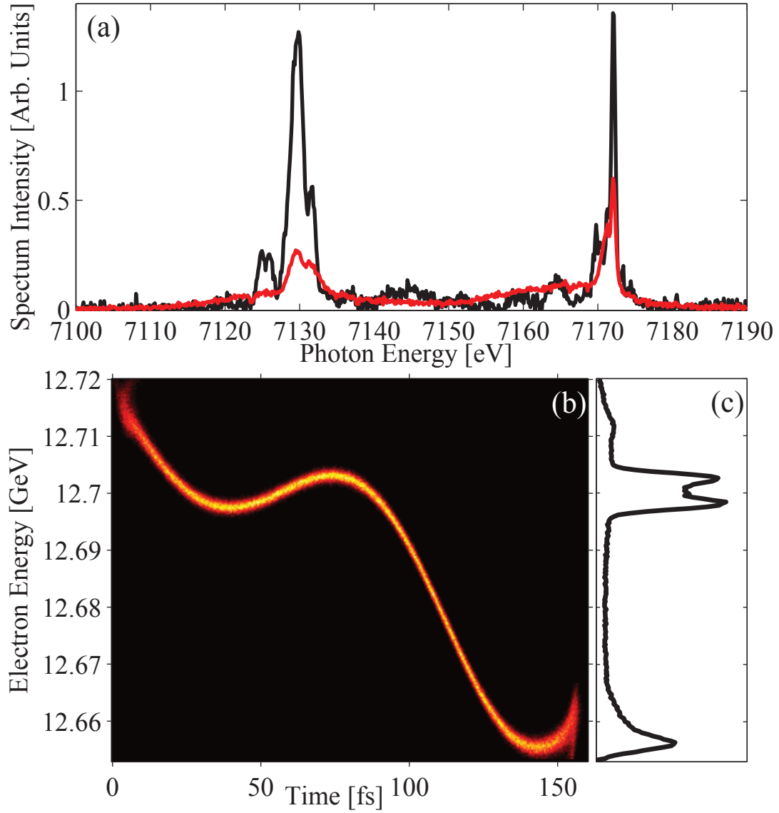
FIG. 5. (a) two-color self-seeded spectrum obtained by using the (-1,1,3) and (1,-1,3) reflections, single-shot (black), average on 100 shots (red). The two color lines are separated by 43 eV ( \sim 0.6\% ) which is wider than the SASE bandwidth for the normal electron beam used in the LCLS. The pulse energy for the shot was 120\mu\text{J} . (b) LiTrack simulated phase space obtained by manipulating the X-band linearizer. (c) Electron beam energy profile for the simulated electron beam, with two energy levels.
