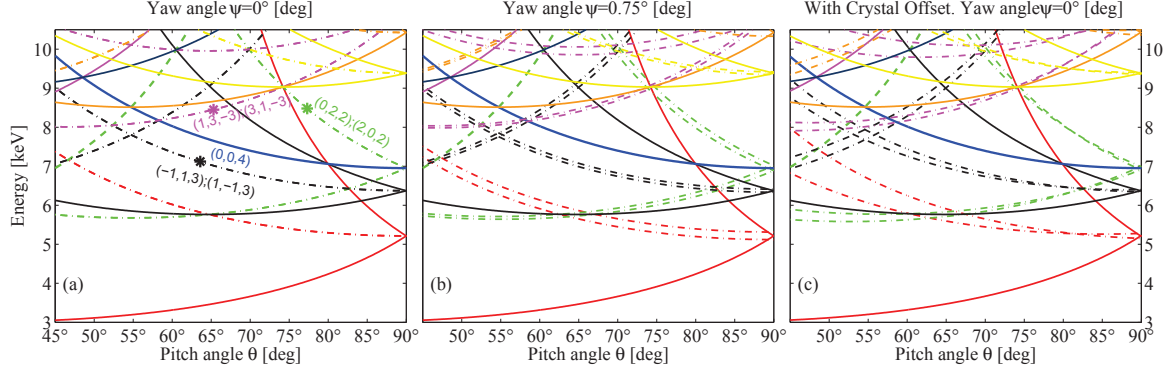
FIG. 2. Photon energy values at which diffraction occurs in a diamond crystal, as a function of the pitch angle \theta for fixed values of yaw angle \psi . Each curve corresponds to reflection from a different set of crystallographic planes. (a) Yaw angle \psi = 0^\circ . Stars represent two-color working points demonstrated in this Letter. (b) Yaw angle \psi = 0.75^\circ . Different colors represent planes with different h^2 + k^2 + l^2 value. Dash-dotted lines are double-lines (two sets of crystal planes excited) that are superposed for \psi = 0^\circ and can be separated with a non-zero yaw angle. (c) Correcting for the small crystal orientation offset deduced from experimental measurements of the energies as a function of (\theta, \psi) values.
