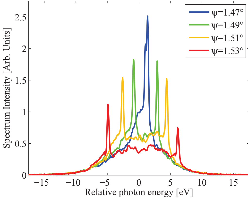
FIG. 3. Average spectra from 111 consecutive shots for single-crystal two-color self-seeded beams with photon energy close to 8.43 keV. The pitch angle was fixed to \theta = 65.28^\circ . (blue) yaw angle \psi = 1.47^\circ . (green) \psi = 1.49^\circ . (orange) \psi = 1.51^\circ . (red) \psi = 1.53^\circ . The used reflection planes were (-1,-3,3) and (-3,-1,3) . The average spectra are shown without post-processing, including the SASE pre-pulse. the plateau between the two narrow colors is mainly due to the wide-bandwidth head part amplified in the second undulator section.
