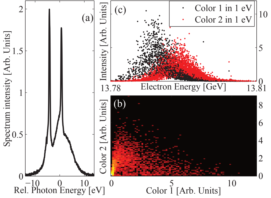
FIG. 4. Single-crystal two-color self seeding experimental results for 3500 consecutive shots. Photon energy was close to 8.43 keV, the reflections used were (2,0,2) and (0,2,2). (a) Average spectrum. (b) Correlation between the first and second color intensities in a 1 eV bandwidth around each color average peak position. (c) Single-shot intensities in a 1 eV bandwidth for both colors vs electron beam energy, (black) color 1; (red) color 2.
