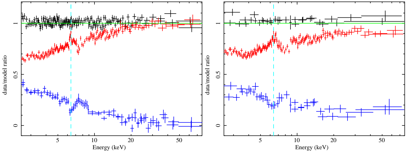
FIG. 10.— Left: The ratios of the interval 2 (black, top), interval 4 (red, middle), and difference (blue, bottom) spectra to the best-fit model to interval 2. Right: The ratios of the interval 6 (black, top), interval 4 (red, middle), and difference (blue, bottom) spectra to the best-fit model to interval 6. Notice the narrow dip in both difference spectra at the energy of neutral Fe K\alpha (6.4 keV as indicated with a dashed, light blue line). XIS-FI, XIS-1, FPMA, and FPMB spectra are shown although only NuSTAR data is shown above 9 keV and only Suzaku data is below 9 keV for clarity. Spectra have been rebinned for plotting purposes only. The solid green line indicates a data/model ratio of unity. (A color version of this figure is available in the online journal.)
