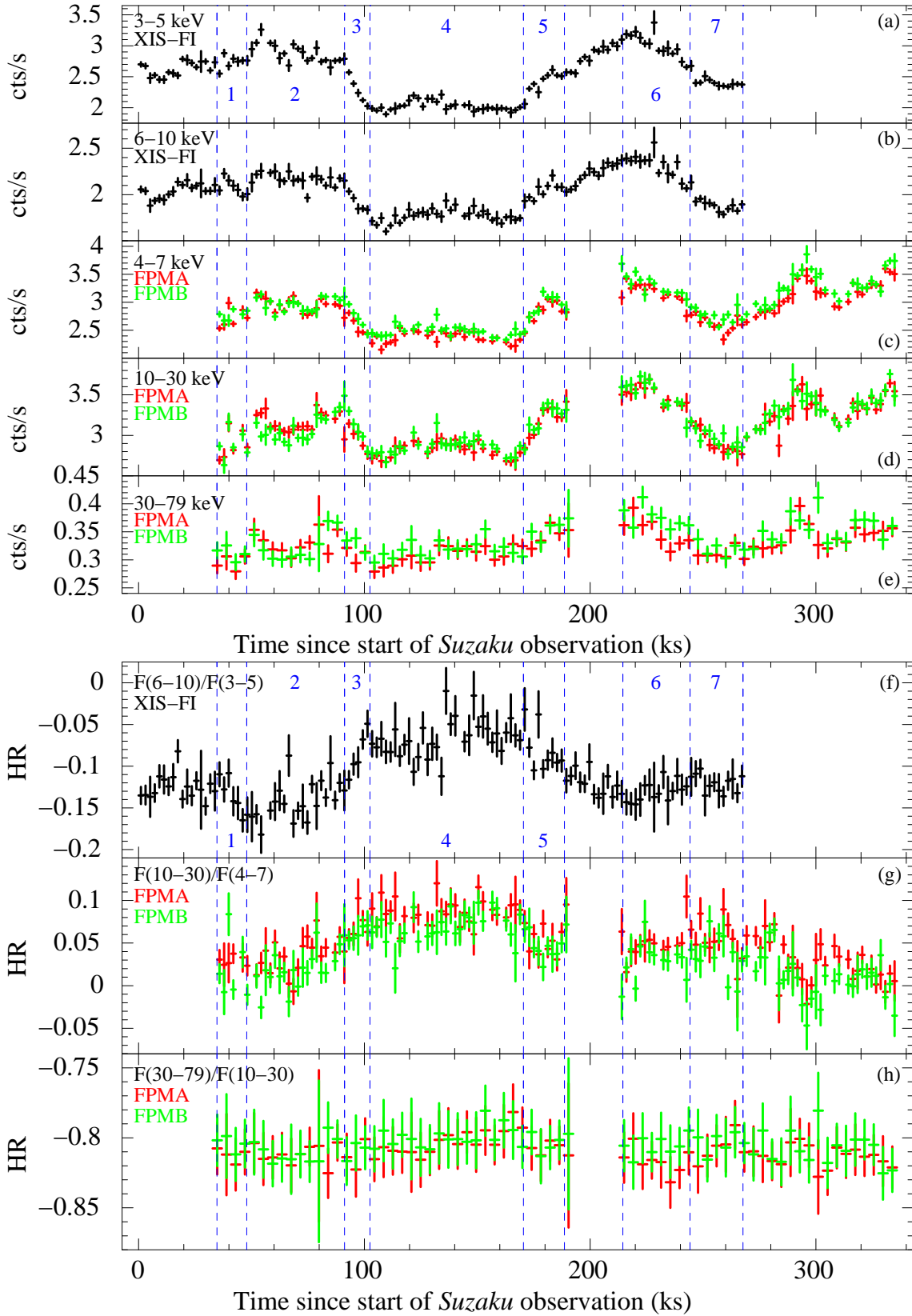
FIG. 2.— Light curves and hardness ratios with 2048 s bins (except for panels (e) and (h), which are shown with 4096 s bins to better show the variability of the 30–79 keV flux). Note the reduction in the broad-band flux coincident with a general increase in spectral hardness seen during a \Delta t \sim 15 ks period labelled interval 3. Panels (a) and (b) show the Suzaku XIS-FI 3–5 keV and 6–10 keV light curves as labelled. Panels (c), (d), and (e) show NuSTAR light curves in the 4–7 keV, 10–30 keV, and 30–79 keV bands, respectively. Panels (f), (g), and (h) show the hardness ratios F(6-10)/F(3-5) , F(10-30)/F(4-7) , and F(30-79)/F(10-30) , respectively. Vertical, blue dashed lines indicate time intervals 1–7 analyzed in the time-resolved analysis as numbered. (A color version of this figure is available in the online journal.)
