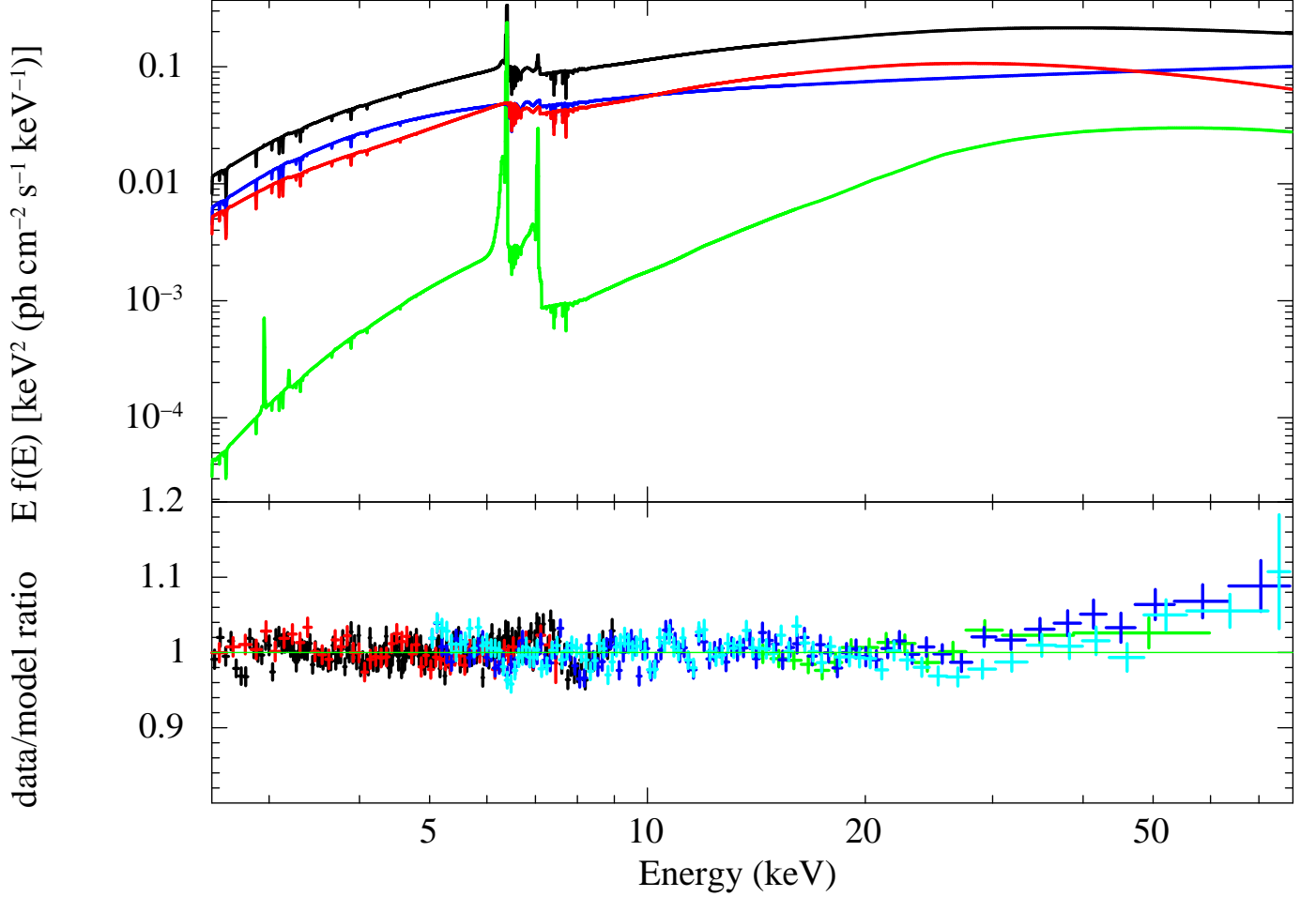
FIG. 5.— Top Panel: Model plotted in Ef(E) . The components are, from top to bottom, the total model (black), the cut-off power-law (dark blue), the inner disk reflection component (red), and the distant reflector component (green). Bottom Panel: The data/model ratios for XIS-FI (black), XIS-1 (red), PIN (green), FPMA (dark blue), and FPMB (light blue). The green line indicates a data/model ratio of unity. For plotting purposes only, spectral bins have either a significance of 80\sigma or a maximum of 80 spectral channels. (A color version of this figure is available in the online journal.)
