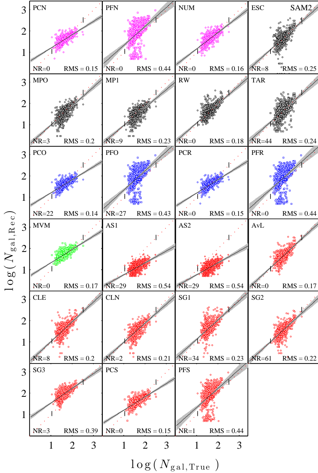
Figure 13. Recovered versus true cluster richness for the 23 methods run on the SAM2 input catalogue. This Figure follows the same notation as in Figure 12.
