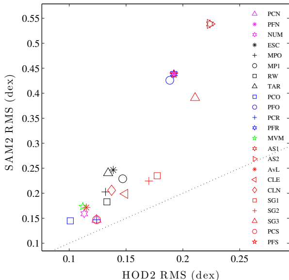
Figure 14. RMS cluster richness errors from the 23 methods applied to the SAM2 input catalogue versus those found when applied to the HOD2 input catalogue. The dotted black line represents a 1:1 relation.
