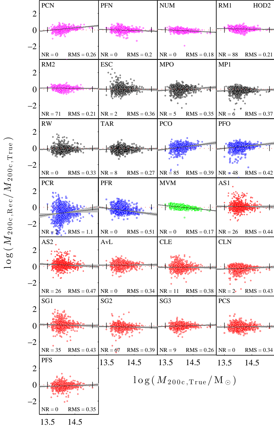
Figure E1. Residuals of the recovered versus true cluster mass for the 25 methods using the HOD2 input catalogue. This Figure follows the same notation as in Figure 2.
