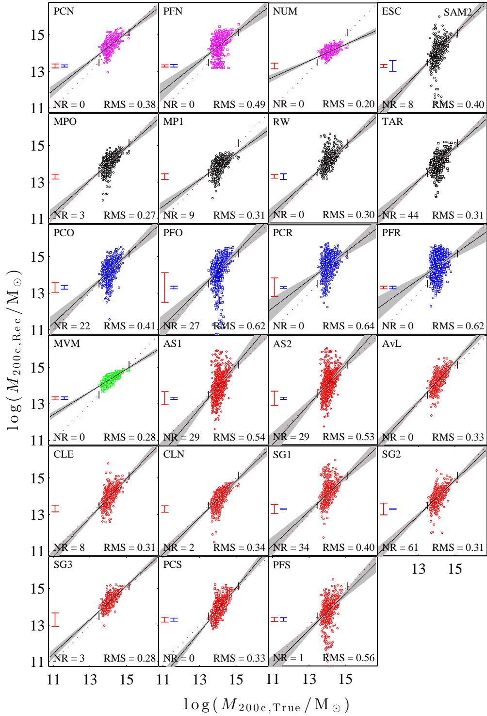
Figure 4. Recovered versus true cluster mass for the 23 methods applied to the SAM2 input catalogue. Same notation as in Figure 2.
