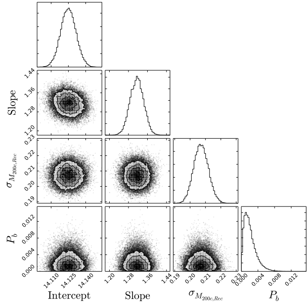
Figure 1. Example of the marginalised probability distributions produced by our MCMC analysis of the PCN method using the HOD2 catalogue for the parameters: the slope ( m ), the intercept ( c ), the scatter in the recovered mass ( \sigma_{M_{\text{Rec}}} ) and the posterior fraction of data points belong to the ‘bad’ outlier distribution ( P_b ).
