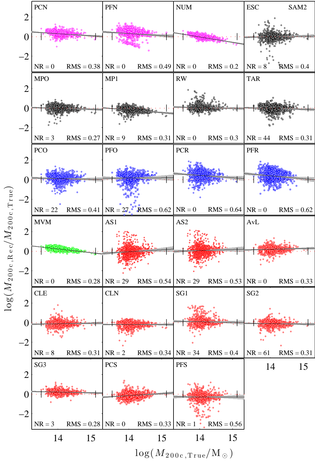
Figure E2. Residuals of the recovered versus true cluster mass for the 23 methods applied to the SAM2 input catalogue. This Figure follows the same notation as in Figure E1.
