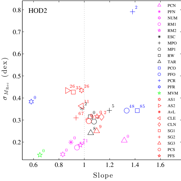
Figure 7. Scatter in the recovered cluster mass versus the slope of the fit to the recovered log mass, both delivered by the likelihood analysis, for the 25 methods applied to the HOD2 input catalogue. The dotted black line identifies a slope of unity. The number next to each methods' marker represents the number of groups/clusters that are not recovered because they are found to have very low ( < 10^{10} M_{\odot} ) or zero mass.
