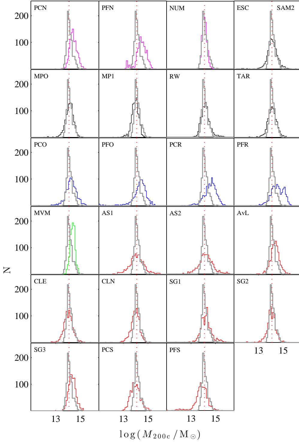
Figure E4. Recovered mass distributions for the 23 methods applied to the SAM2 input catalogue. This Figure follows the same notation as in Figure E3.
