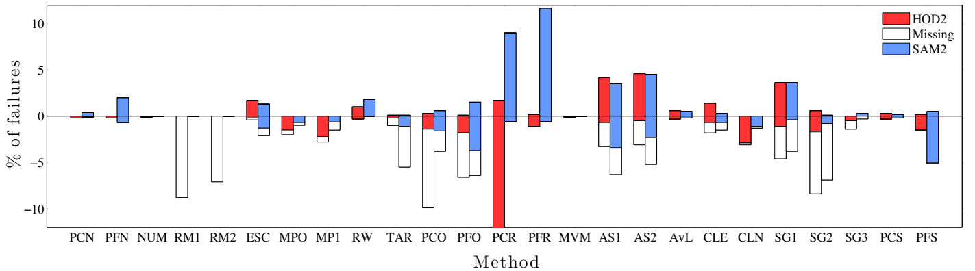
Figure 11. Histogram of the percentage of groups/clusters whose recovered mass is over-estimated (positive %) or underestimated (negative %) by a factor of ten or more relative to the true mass for all methods applied to the HOD2 (red) and SAM2 (blue) input catalogues. The white segments of each bar represents the number of missing groups/clusters. Note that the y-axis of this plot is truncated so that detail at the low percentage range is seen more clearly. PCR falls below this truncation with 32.1% of group/cluster masses underestimated by a factor of ten.
