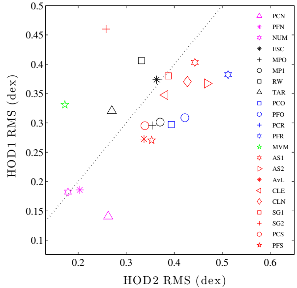
Figure 3. RMS cluster mass accuracies with the simple HOD1 input catalogue versus those derived from the more sophisticated HOD2 catalogue. The dotted black line represents a 1:1 relation. Note: PCR lies beyond the axes of this figure with an RMS of 1.07 dex for HOD2 and 0.74 dex for HOD1.
