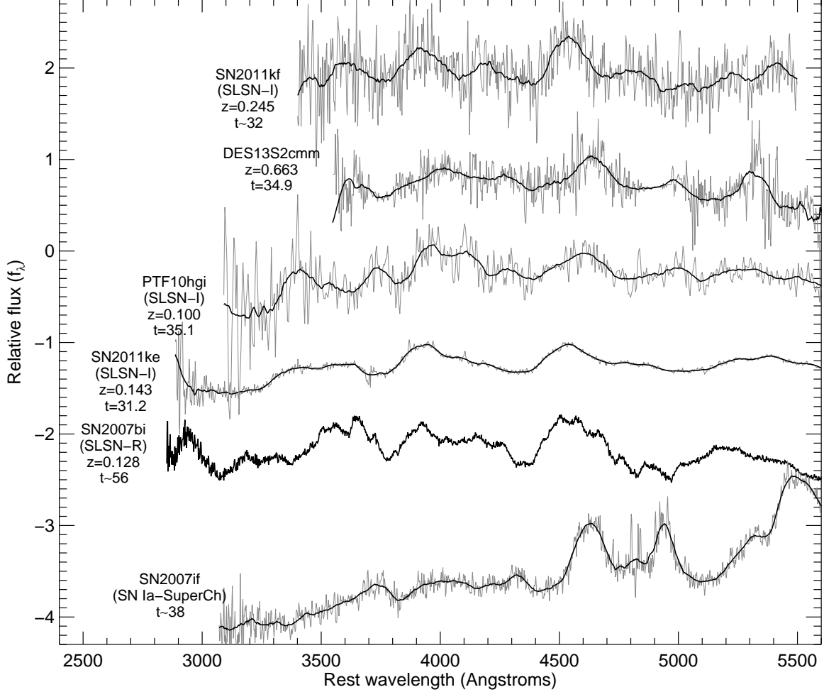
Figure 4. The VLT FORS2 spectrum of DES13S2cmm (second from top) compared to other SLSNe of similar phase in their light curves. From top to bottom, we also show SN 2011kf (Inserra et al. 2013), PTF10hgi (Quimby et al. 2011), SN 2011ke (Inserra et al. 2013) and SN 2007bi (classified as Type R in Gal-Yam et al. 2009); as discussed in Section 3.2, SUPERFIT identifies these SLSNe as some of the best-fitting spectral templates to DES13S2cmm. In each case, the light grey shows the raw data and the solid line is a Savitsky-Golay smoothed version of the spectrum. The spectra are labelled with the SN name, SLSN type (except DES13S2cmm), redshift, and the phase when the spectrum was taken. We show the spectrum of the ‘super-Chandrasekhar’ SN Ia SN 2007if as discussed in Scalzo et al. (2010). Note that the spectrum for 2007bi, while at a later phase than the other data, is the earliest spectral observation of this SN.
