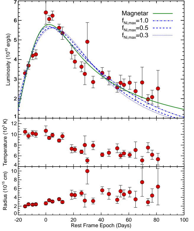
Figure 6. Upper panel: Bolometric light curve of DES13S2cmm, with the best-fit magnetar model (green solid line) and three ^{56}\text{Ni} models with different f_{\text{Ni,max}} (blue lines) overplotted. The magnetar model is a better match to the data than the best-fit ^{56}\text{Ni} , and has a significantly better \chi^2 than the models with a more realistic f_{\text{Ni,max}} (see text). However both models have difficulty reproducing the peak luminosity, the post-peak decline, and the late-time flattening. Middle and Bottom panels: Temperature and radius evolution of the best-fitting blackbody to each photometric epoch which is used to construct the bolometric light curve.
