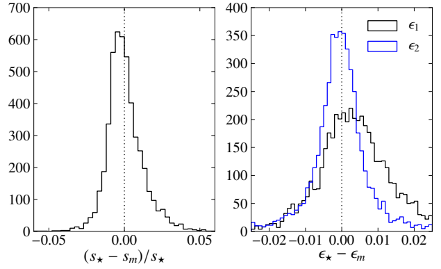
Figure A1. Fractional size and ellipticity residuals of the PSFEx model shown in Figure 3 but for a set of stars with \text{MAG\_AUTO} \in [15, 21.5] . The brighter stars in this selection lead the PSF model to adopt larger sizes and a preferred \epsilon_1 -direction, which is not shared by the bulk of the (fainter) stars.
