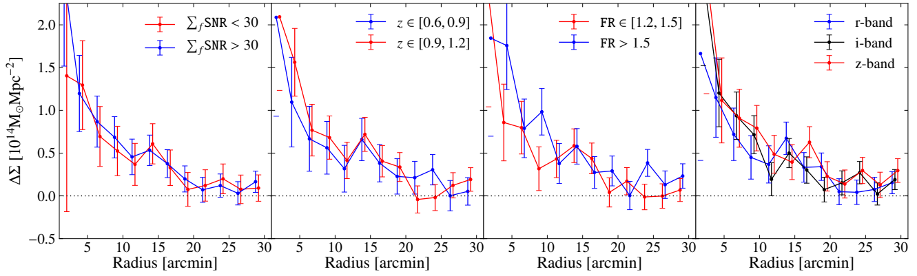
Figure 5. Consistency test for the background-selected shape catalogs, sliced in IM3SHAPE’s \Sigma_f SNR ( 1st panel ), in photo- z estimate ( 2nd panel ), in FWHM_RATIO (FR for short, 3rd panel ), and from different filters ( 4th panel ). The conversion between shear estimate and \Delta\Sigma is done with \Sigma_{\text{crit}}(z) calculated for each galaxy individually based on its photometric redshift according to Equation 8. The numbers are stacked over the four fields, errors correspond to the dispersion of the weighted mean in each bin. For clarity, the points of different slices have been shifted horizontally by 0.4 arcmin.
