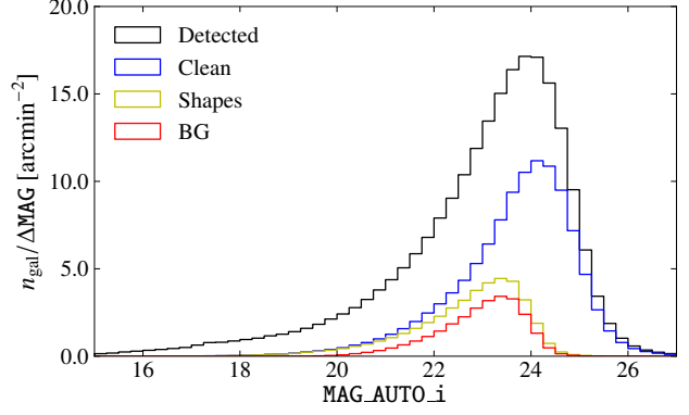
Figure 1. Galaxy number density n_{\text{gal}} in bins of SECTOR’s magnitude \text{MAG\_AUTO}_i in the i -band. From top to bottom: detected sources (black); after cleaning the catalog (blue); galaxies with successful shape measurements (yellow); galaxies considered in the lensed background sample (red). See Section 4.3 for details on the selections. The numbers are unweighted, averaged over all four fields.
