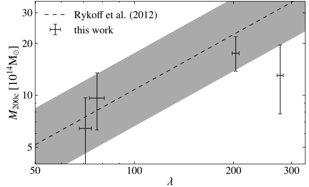
Figure 7. Lensing mass M_{200c} as a function of redMaPPer's richness \lambda for the four investigated clusters. The dashed line shows the expected scaling relation from Rykoff et al. (2012, see Equation 18) with their proposed relative scatter of 33% at fixed richness ( shaded region ).
