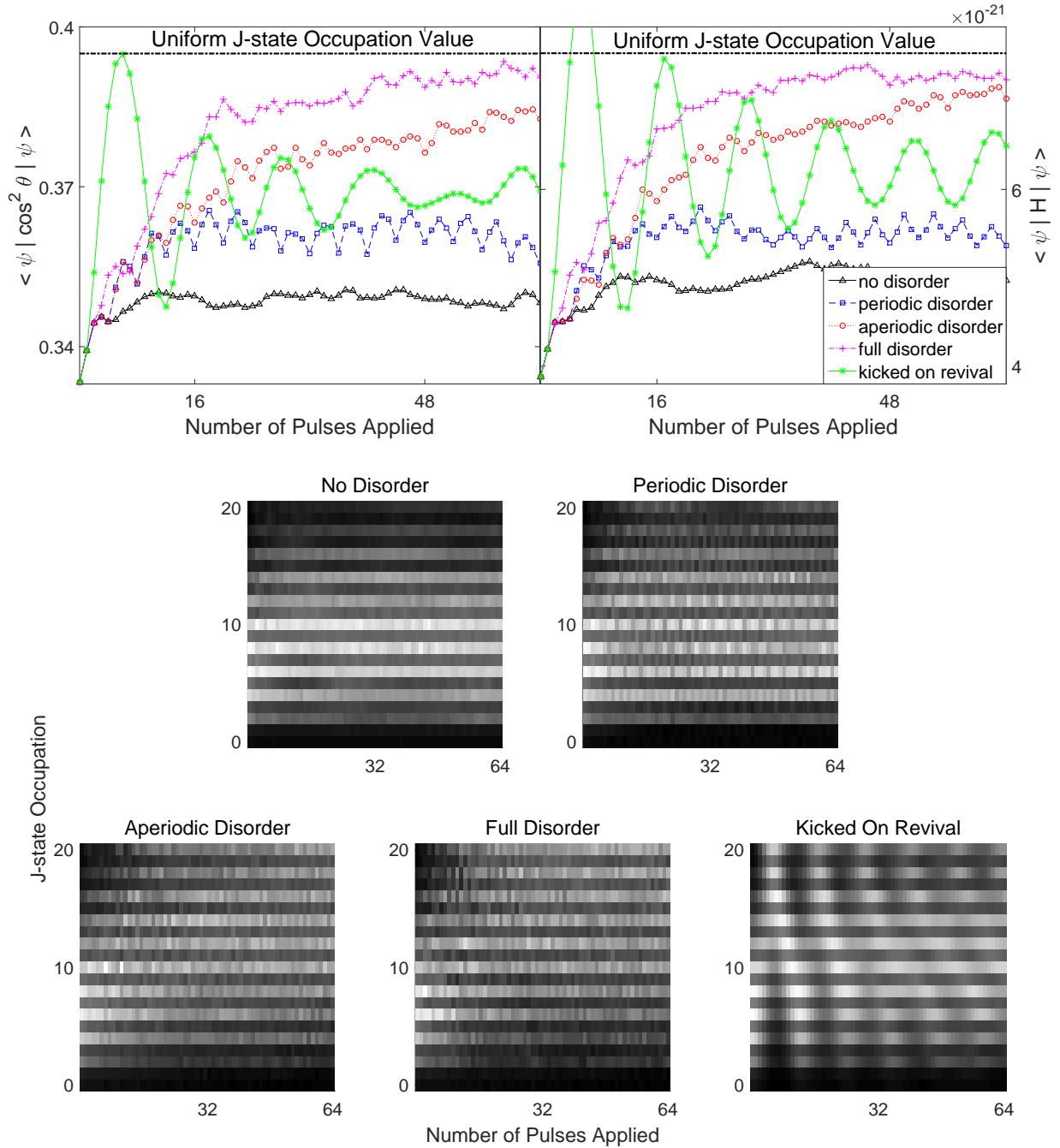
FIG. 1. Simulated population alignment and energy for extended pulse trains with different levels of spacing disorder. The train with no disorder is a pulse train with uniform \tau = 1.159T_{rev} = \frac{2\pi+1}{2\pi}T_{rev} . The periodic disorder train consists of a repeating series with three spacings of \tau = 1.159T_{rev} and a fourth spacing of \tau = 1.183T_{rev} . The aperiodic disorder train is similar to the periodic sequence, except every fourth spacing is a randomly generated value within the range \tau = [1.159T_{rev}, 1.207T_{rev}] . The full disordered train uses random values within the range \tau = [1.159T_{rev}, 1.207T_{rev}] for all spacings. The train that excites ^{14}\text{N} with kicks on revival is periodic with all \tau = T_{rev} ; it is plotted here for reference only. The rotational energy of ^{14}\text{N} is plotted for comparison to theoretical studies of dynamical localization. The relationship between these two values is not one-to-one but shows matching behaviors, especially in terms of boundedness. The color maps indicate the J-state population distribution as a function of kick count for each of the applied pulse trains. The peak intensity used for this simulation is 1.2 \cdot 10^{14} \frac{\text{W}}{\text{cm}^2} . T_{rev} is the well known ^{14}\text{N} alignment revival time of 8.38 ps.
