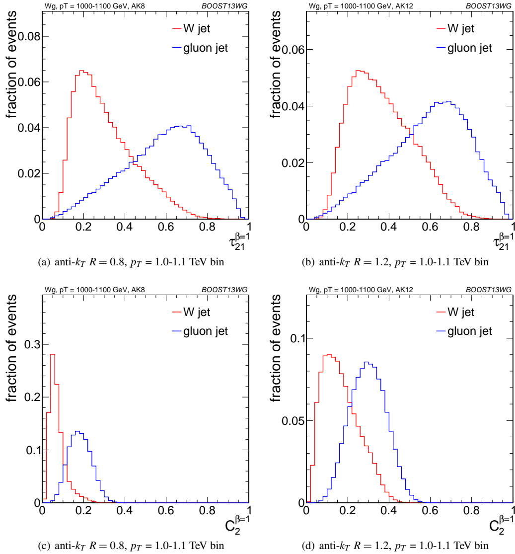
Fig. 21 The \tau_{21}^{\beta=1} and C_2^{\beta=1} distributions for signal and background R = 0.8 and R = 1.2 jets in the p_T = 1.0-1.1 \text{ TeV} bin.
