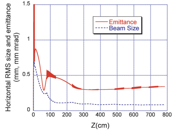
Figure 3: PARMELA simulation of the rms horizontal beam size and emittance in the photoinjector and linac
