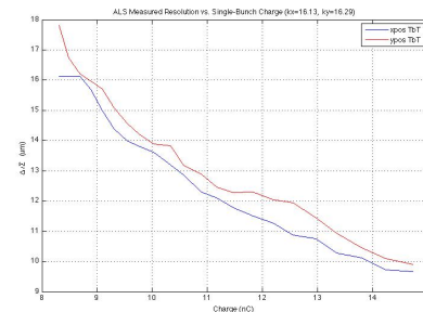
Fig. 3: Measured Resolution vs. Charge
