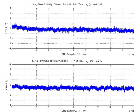
Fig. 7: Measured Long-Term Stability
