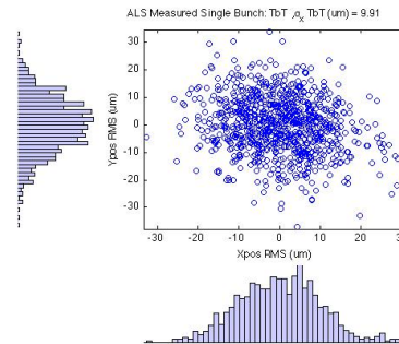
Fig. 2: Single Bunch TbT Scatter-Histogram
