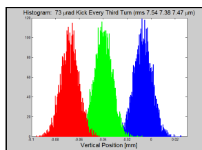
Fig. 6: Orbits kicking every 3 rd turn
