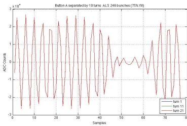
Fig. 4: 246-Bunch 75% Fill Single Turn
