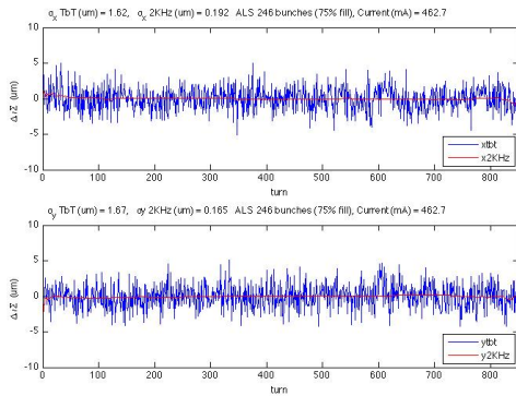
Fig. 5: 246-Bunch TbT and 2KHz Resolution
