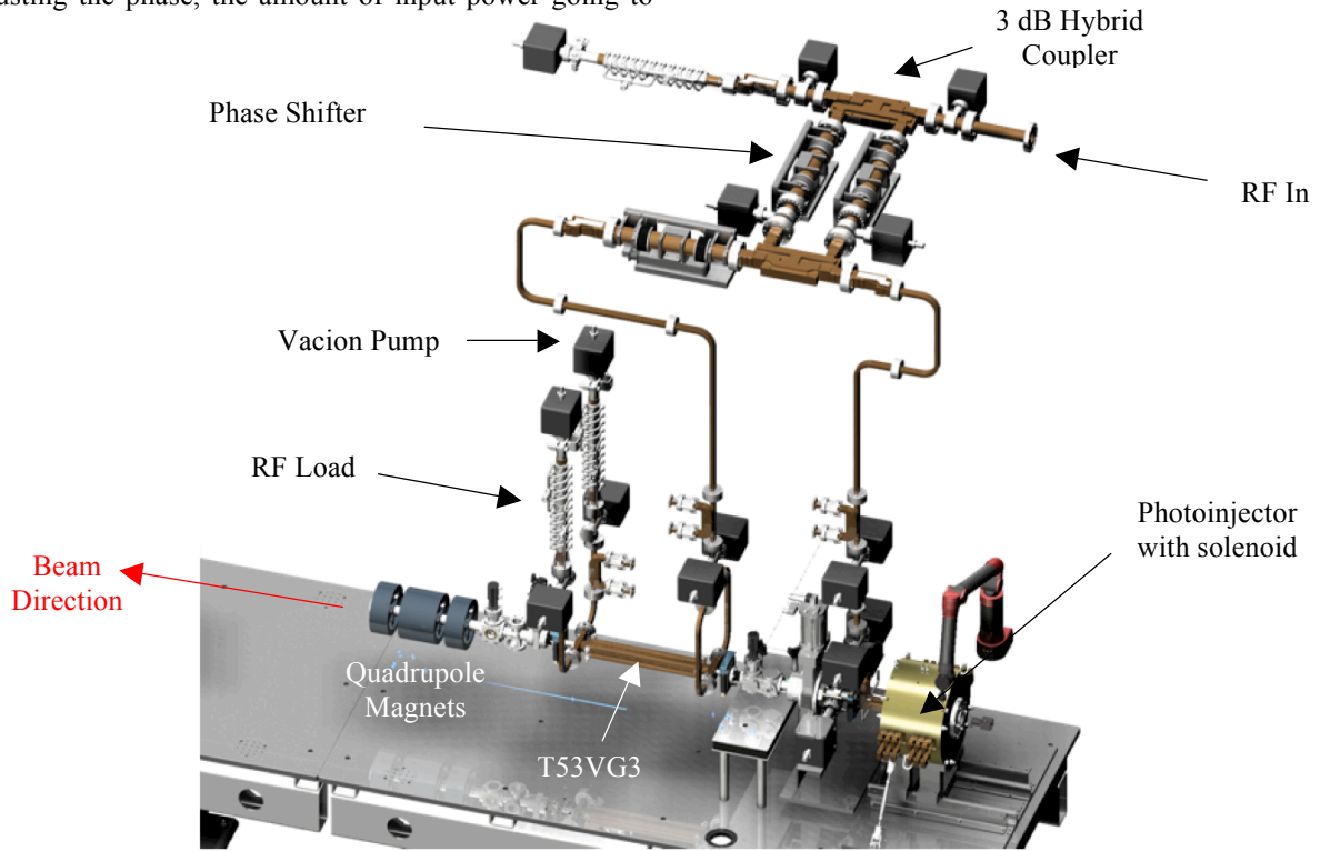
Figure 3. Illustration of RF distribution at photoinjector.
