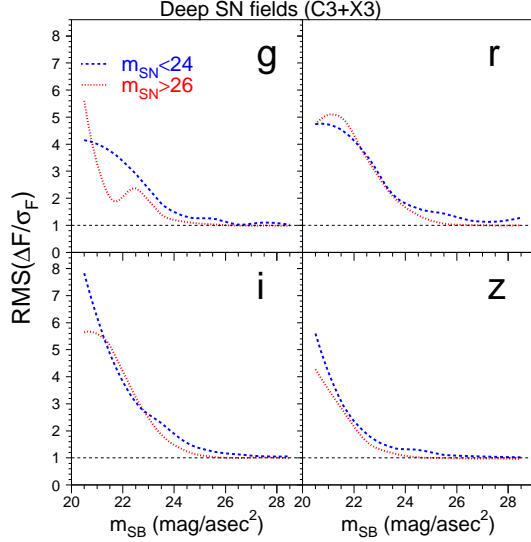
FIG. 9.— For the 2 deep fields in each pass band, RMS of \Delta F/\sigma_F as a function of the galaxy surface-brightness mag ( m_{SB} ) for fakes as defined in the text. \Delta F is the difference between the true and measured fake flux, and \sigma_F is the uncertainty. The horizontal dashed line through 1 shows the expected value if DiffImg correctly determines the flux uncertainties. The dotted-red curve is for very faint fakes with SN mag m > 26 ; the dashed-blue curve is for fakes with SN mag m < 24 . The model for this effect (§5) depends on m_{SB} and not on the transient mag.
