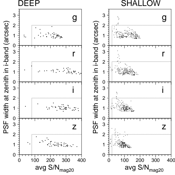
FIG. 5.— For each set of exposures in Y1, the CCD-averaged PSF width ( i -band at zenith, FWHM, arcsec) is plotted against the CCD-averaged S/N from the MAG20 fakes. Exposure sequences with points outside the dashed box are retaken, typically the following night. Left panels are for the deep-fields and the right panels are for the shallow fields.
