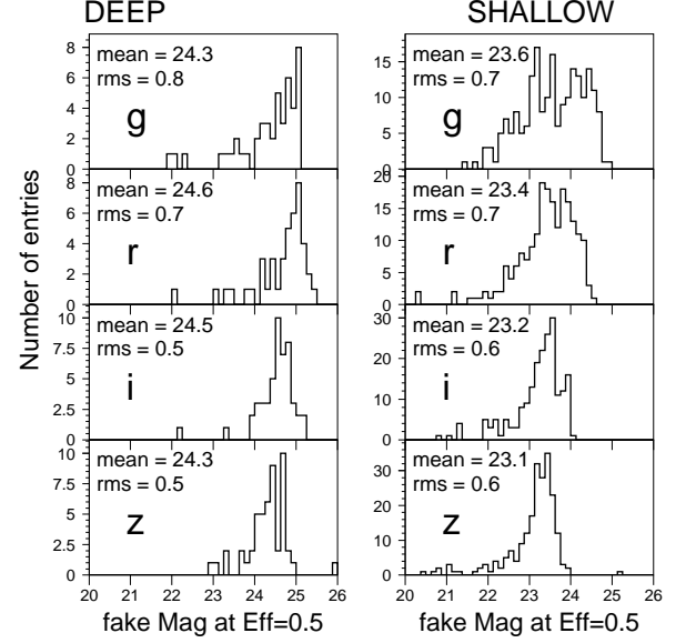
FIG. 7.— Distribution of m_{\text{eff}}=1/2 in each passband, determined with fakes. Each entry is from one epoch. Left panels are for the deep fields; right for the shallow fields.
