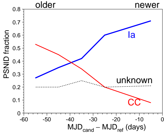
FIG. 4.— PSNID classification fraction for SN Ia and SN CC vs. time that the light curve has been observed, for candidates in which three bands have an observation with S/N > 5 . See §3.6 for explanation of MJD_{\text{cand}} and MJD_{\text{ref}} . Zero on the horizontal axis corresponds to newer candidates used in the PSNID fits; -50 days corresponds to older candidates whose second detection occurred 50 days earlier and thus have longer light curve coverage in the PSNID fits. “Unknown” corresponds to light curves for which PSNID cannot determine a SN type.
