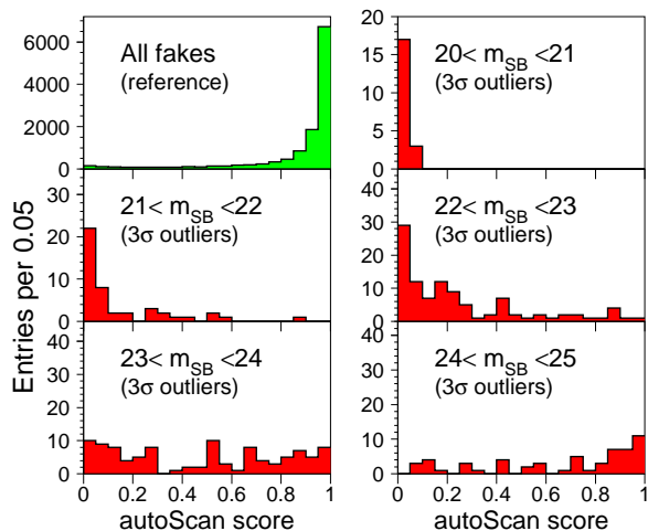
FIG. 14.— autoScan score distribution for fakes in the two deep fields, i band. Score is 0 for a clearly bad subtraction and 1 for a good subtraction. Upper left panel shows the reference distribution for all fakes. Remaining panels probe the SB anomaly for a subset of fakes that are faint ( m_{\text{SN}} > 23 ), are detected by SExtractor , satisfy the cuts in Table 3, and have a measured flux more than 3\sigma away from the true flux. Each panel indicates a different m_{\text{SB}} range.
