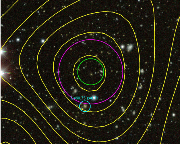
Figure 6. SPT-CL J0433-5630: DES-SVA1 gri pseudo colour image overplotted with SPT-SZ signal-to-noise contours (in steps \Delta\xi=1 ). The magenta circle shows the projected R_{500}/2 radius at z = 0.69 , while the green circle describes the 1\sigma SPT positional uncertainty (Eq.11). The cyan label marks the associated \lambda \sim 60 RM cluster.
