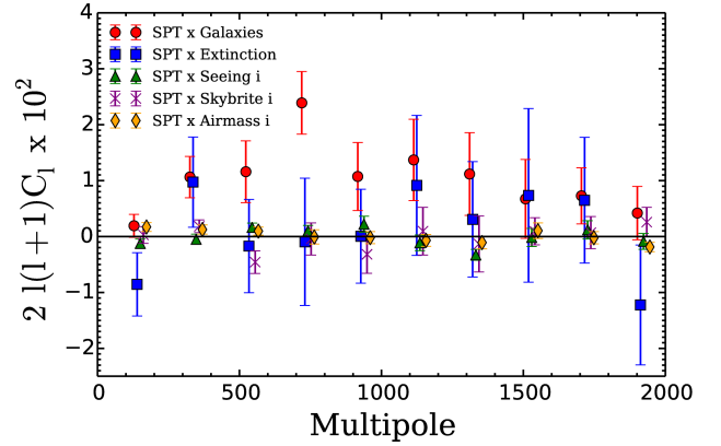
Figure 18. Correlations between the SPT convergence map and the potential systematics maps. Data points are offset on the x -axis for clarity. The galaxy-lensing correlation ( red circles ) is detected at 6\sigma , while the majority of the SPT cross systematic maps data points are consistent with zero. Correlating the SPT maps with DES potential systematic maps is expected to produce a null result, which we recover.
