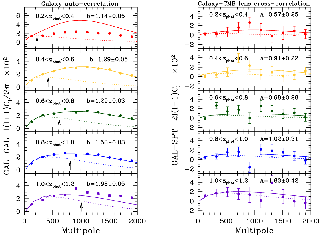
Figure 11. Harmonic space redshift tomography of the auto- (left column) and cross- (right column) correlations. The panels from top to bottom describe the results of photo- z bins of increasing redshift. The solid lines show our fiducial cosmology rescaled by the best-fit linear bias b up to weakly non-linear scales \ell_{\text{NL}} marked with an arrow (for the auto-spectra) or the cross-correlation amplitudes A = bA_{\text{Lens}} over the whole range of scales (cross-spectra); the best-fit biases and amplitudes are reported in the captions with their 1\sigma errors. The dotted lines are linear theory predictions, and the error bars are from the full N -body covariance estimator. In agreement with the real-space analysis and with Crocce et al. (2016), the auto-correlation in the lowest (and less significantly in the highest) redshift bins does not match the theoretical expectation on non-linear scales, which are discarded from our bias fits anyway.
