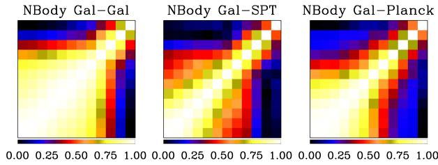
Figure 6. Correlation matrices for the three cases we consider, estimated with the N -body method. The matrices refer to galaxy-galaxy, galaxy-SPT, and galaxy-Planck lensing respectively. The angular range is from 2.4 arcmin to 5 deg as in Fig. 5. We see that the galaxy-CMB lensing correlation matrix is more diagonal than the galaxy-galaxy case, as the auto-correlation theory is more non-linear, and thus more non-Gaussian and less diagonal. Furthermore, all matrices become less diagonal in the first few angular bins due to the introduction of the Gaussian smoothing to the maps, which effectively blurs information on scales \theta < \theta_{\text{FWHM}} = 5.4' (DES-SPT) and 10.8' (DES-Planck).
