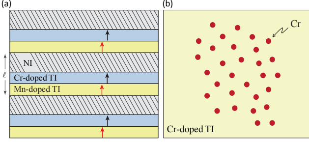
FIG. 1. (color online). Schematic drawing of the proposed systems to realize the dynamical axion field. (a) The magnetic TI superlattice structure. The upper and lower halves of TI films are doped with Cr and Mn, respectively. The arrows in TI layers indicate the magnetization direction. In each crystalline unit cell, the z -direction thickness of Mn-doped TI, Cr-doped TI, and NI layers are \ell_m , \ell_c , and \ell_n . (b) Topological PM insulator: 3D TI materials close to topological QCP doped with Cr, where a PM state is realized.
