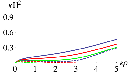
FIG. 6. Graphical representation of \kappa H^2 as a function of \kappa\rho for a radiation dominated universe ( w = 1/3 ) with \beta > 1/4 and \kappa being positive. The solid blue, red, and green curves represent the solutions for \beta = 7/10 , 4/5 , and 9/10 , respectively. The dashed blue, red and green curves represent the solutions for \beta = 19/20 , \beta = 1 and \beta = 6/5 , respectively.
