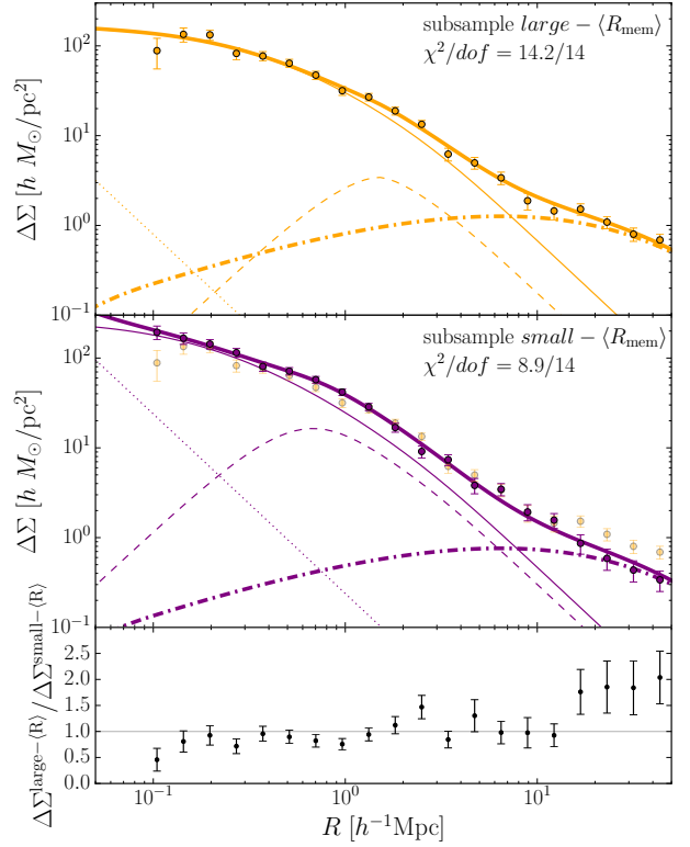
FIG. 1. Halo mass consistency and assembly bias from the WL signal.: The data points with errorbars in the top and middle panels show the excess surface mass density profile as a function of the cluster-centric projected radius (in comoving units), obtained from the WL measurements for the large- and small- \langle R_{\text{mem}} \rangle subsamples of redMaPPer clusters (see Eq. 1), respectively. The points from the top panel are reproduced in semi-transparent color in the middle panel for comparison. The mass profiles at small radii R \lesssim 10 h^{-1}\text{Mpc} appear to have similar amplitudes with slightly different shapes, but show a difference in amplitude at R \gtrsim 10 h^{-1}\text{Mpc} , as expected from assembly bias . The bold solid line shows the best-fit halo model, the thin solid line is the centered 1-halo term, the dashed line is the off-centered 1-halo term, while the dotted line corresponds to the stellar mass contribution from the central galaxy. Comparison between the dot-dashed lines in the two panels implies that the 2-halo term contributions, which arise from the average mass distribution surrounding the clusters, are different by a factor of 1.6. The bottom panel shows the ratios of the lensing signals, highlighting a clear deviation from unity at R \gtrsim 15 \text{ Mpc}/h .
