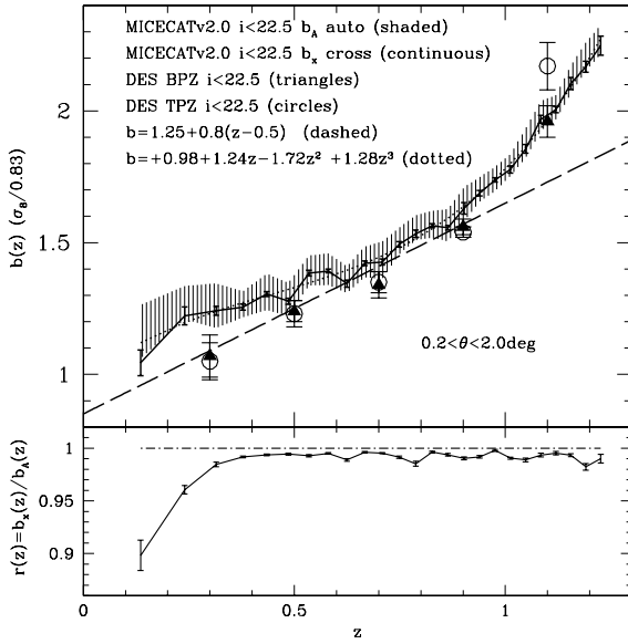
Figure 17. Top panel shows the evolution of galaxy bias with redshift in a flux limited sample ( i < 22.5 ) similar to the one defined in this paper but selected from our MICECATv2.0 mock galaxy catalog. We display bias derived from galaxy auto-correlations b_A = \sqrt{w_{gg}/w_{mm}} and galaxy-matter cross correlation b_X = w_{gm}/w_{mm} . The evolution is similar to the one in the DES-SV data. Bottom panel shows the ratio of the two estimates, i.e. the stochasticity coefficient r = b_A/b_X , which we found close to unity in the redshift range relevant for DES data.
