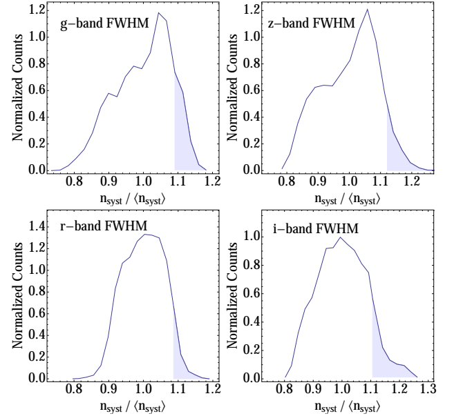
Figure 7. Distribution of FWHM weighted co-added values in different bands across our footprint. The shaded parts of the histograms correspond to regions where large decrement of galaxy density in different photo- z bins is found. To avoid a systematic effect they were removed from the corresponding clustering analysis. See Sec. 6.1 for further details.
