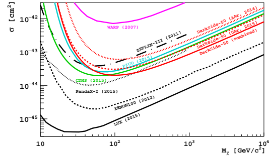
FIG. 5. Spin-independent WIMP-nucleon cross section 90 % C.L. exclusion plots for the DarkSide-50 AAr (dotted red) and UAr campaigns (dashed red), and combination of the UAr and AAr [38] campaigns (solid red). Also shown are results from LUX [58] (solid black), XENON100 [59] (dashed black), PandaX-I [60] (dotted black), CDMS [61] (solid green), PICO [62] (solid cyan), ZEPLIN-III [63] (dash dotted black) and WARP [64] (magenta).
