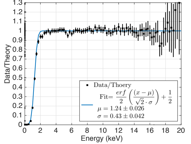
FIG. 6: Ratio of the measured tritium energy spectrum and the true one convolved with the detector resolution. A fit to an error function is shown.
