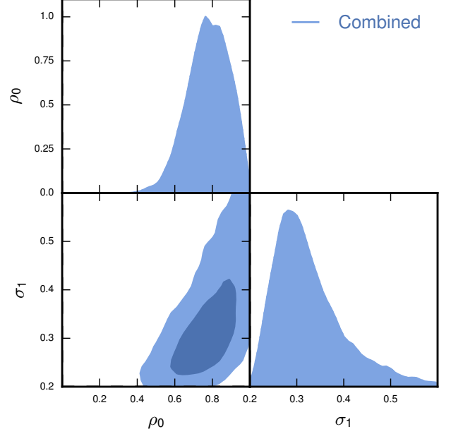
Figure 12. Posterior distribution for the 1\sigma and 2\sigma levels of two of the parameters ( \rho_0, \sigma_1 ) from the positional offset model in Eqn. 4, for the combined XCS, Chandra , and SPT data. Best fit parameters are shown in Table 2. The predicted well-centered fraction determined from redMaPPer centering probabilities is \langle P_{\text{cen}} \rangle = 0.82 , consistent with the best-fit value.
