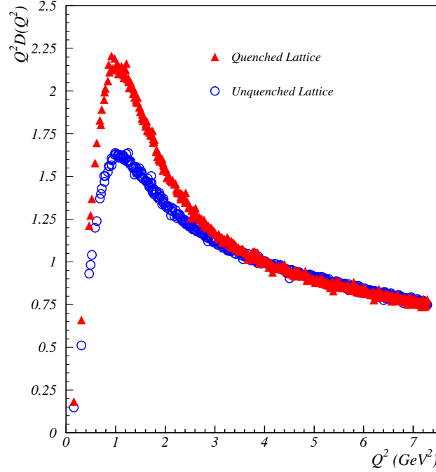
Figure 4.5: The gluon dressing function Z(Q^2) = Q^2 D(Q^2) , from quenched and full lattice calculations from Bowman et al. , Ref. [330].
