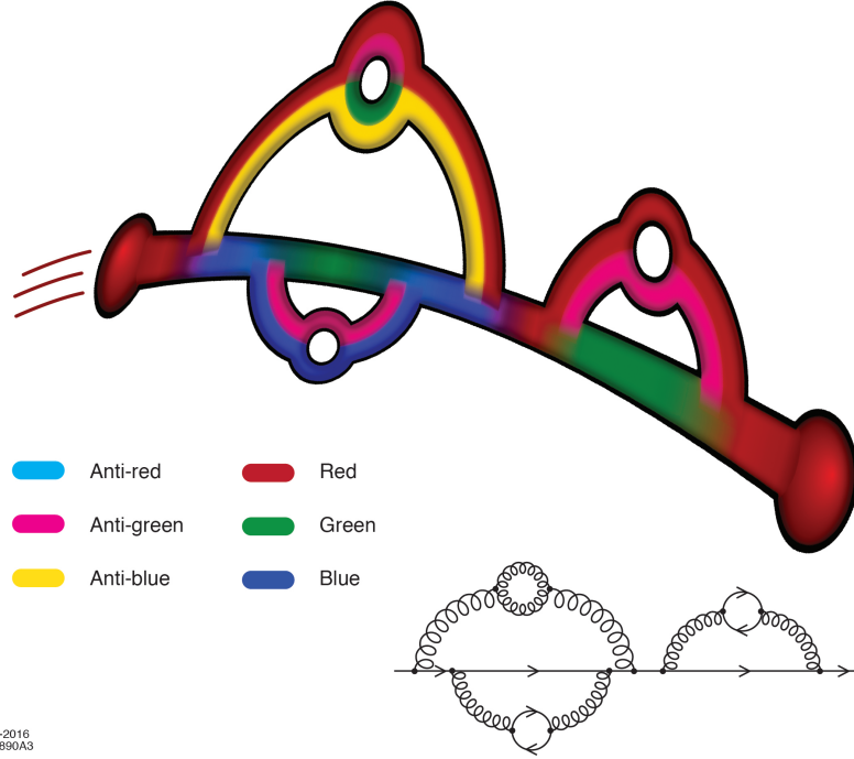
Figure 2.1: (Color online) Color spread and the physics of asymptotic freedom and confinement. In contrast with QED the force carriers of QCD, the gluons, carry color charges which leads to spread of color. The dilution of the initial color charge is responsible for the weakening of the QCD coupling \alpha_s at small distances; i. e. , when the quark experiences a large momentum transfer. Since there is no intrinsic length scale, values of \alpha_s at different momentum transfer scales are related by a logarithmic function: \alpha_s decreases continuously with increasing momentum transfer (shorter distances) leading to asymptotic freedom. Conversely \alpha_s increases logarithmically at larger distances. However, this growth with large distance cannot continue indefinitely since the proton has a finite size: color is confined. Confinement implies that long wavelengths of quarks and gluons are cut off at a typical hadronic size. Consequently, the effects of quantum loops responsible for the logarithmic dependence of \alpha_s disappear and \alpha_s should freeze to a constant value at hadronic scales [5, 6]. The evolution of a quark's color is illustrated in the figure. Here, an initially red quark converts to either a green or blue quark when its red color charge is carried away by the emission of a gluon. The anti-red color is symbolized as cyan, anti-green as magenta and anti-blue as yellow. In the accompanying diagram, the straight line represents a color-triplet quark (or an anti-quark), and a curved line represents a color-octet gluon carrying both color and anti-color.
