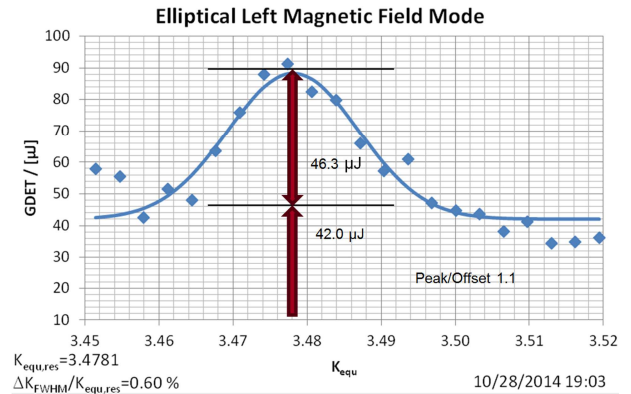
Figure 11: Delta resonance scan in elliptical left magnetic field mode (elliptical right polarization) in regular afterburner configuration.
