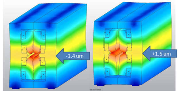
Figure 6: Shape deforming of Delta due to the transverse magnetic forces of \pm 15,000 \text{ N} , according to finite element modelling. Measured values are indicated inside arrows.
