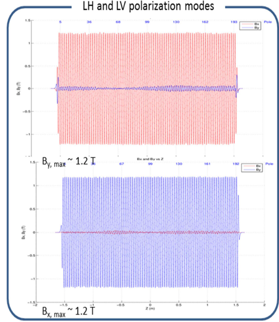
Figure 8: Undulator magnetic fields (red: B_x , blue: B_y ) for the linear horizontal (LH) and linear vertical (LV) polarization modes at maximum K value.
