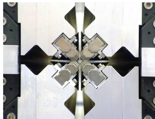
Figure 5: Front view of the fully assembled Delta undulator. Visible are the Al magnet block carriers and part of the precision rail system [6].
