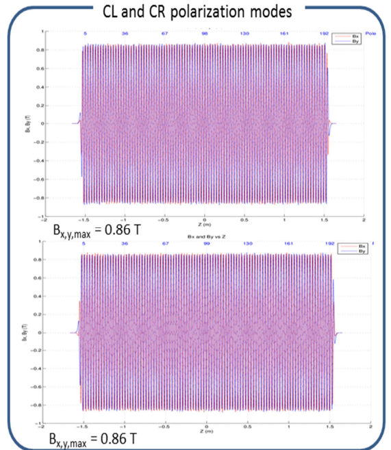
Figure 9: Undulator magnetic fields (red: B_x , blue: B_y ) for the circular left (CL) and circular right (CR) polarization modes at maximum K value.
