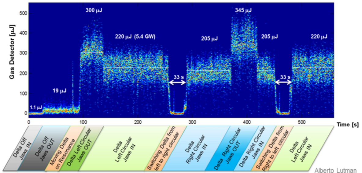
Figure 15: Delta polarization switching during operation.
