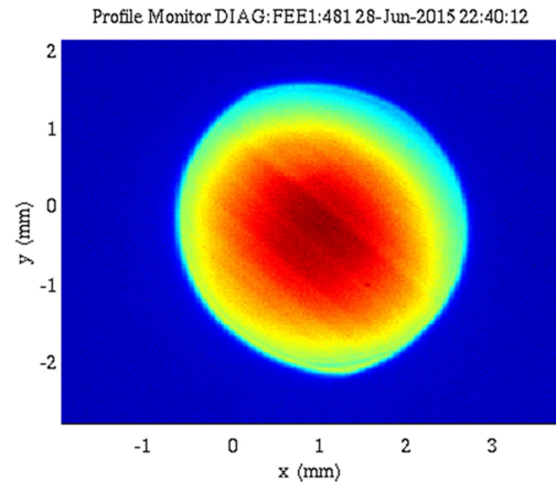
Figure 13: X-ray pulse image at 710 eV on Direct Imager in reverse taper contribution.
