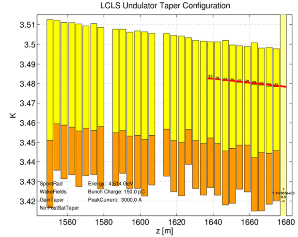
Figure 10: K values of the LCLS micro-bunching undulators segments for Delta operation in regular afterburner mode.
