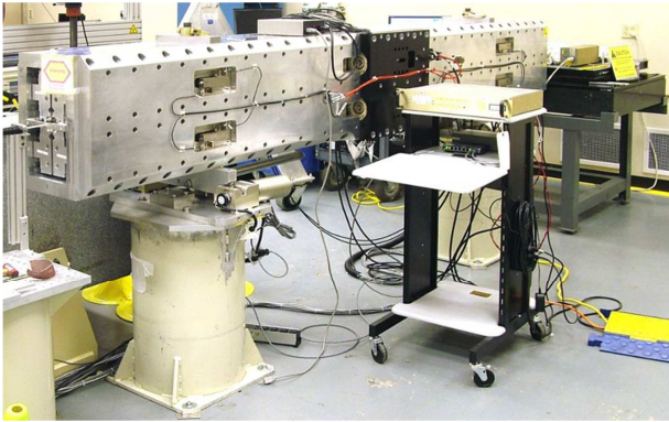
Figure 7: Delta undulator on the field mapping stand.
