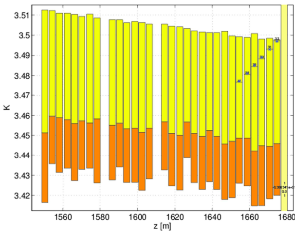
Figure 12: K values of the LCLS micro-bunching undulators segments for Delta operation in reverse taper mode.
