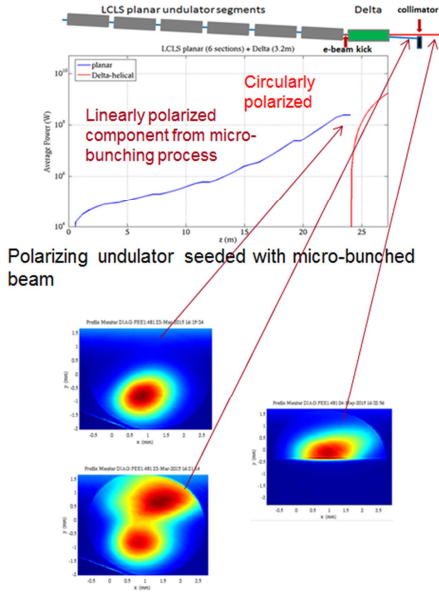
Figure 14: Beam diversion and collimation pushes degree of circular polarization close to 100 %.
