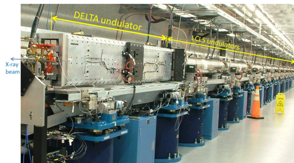
Figure 1: 3.2-m long LCLS Delta undulator installed at the end of the LCLS undulator line.
