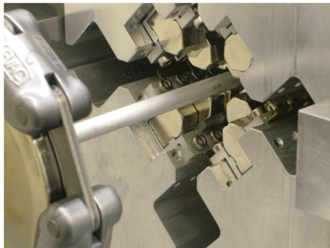
Figure 4: Delta undulator with vacuum chamber.
