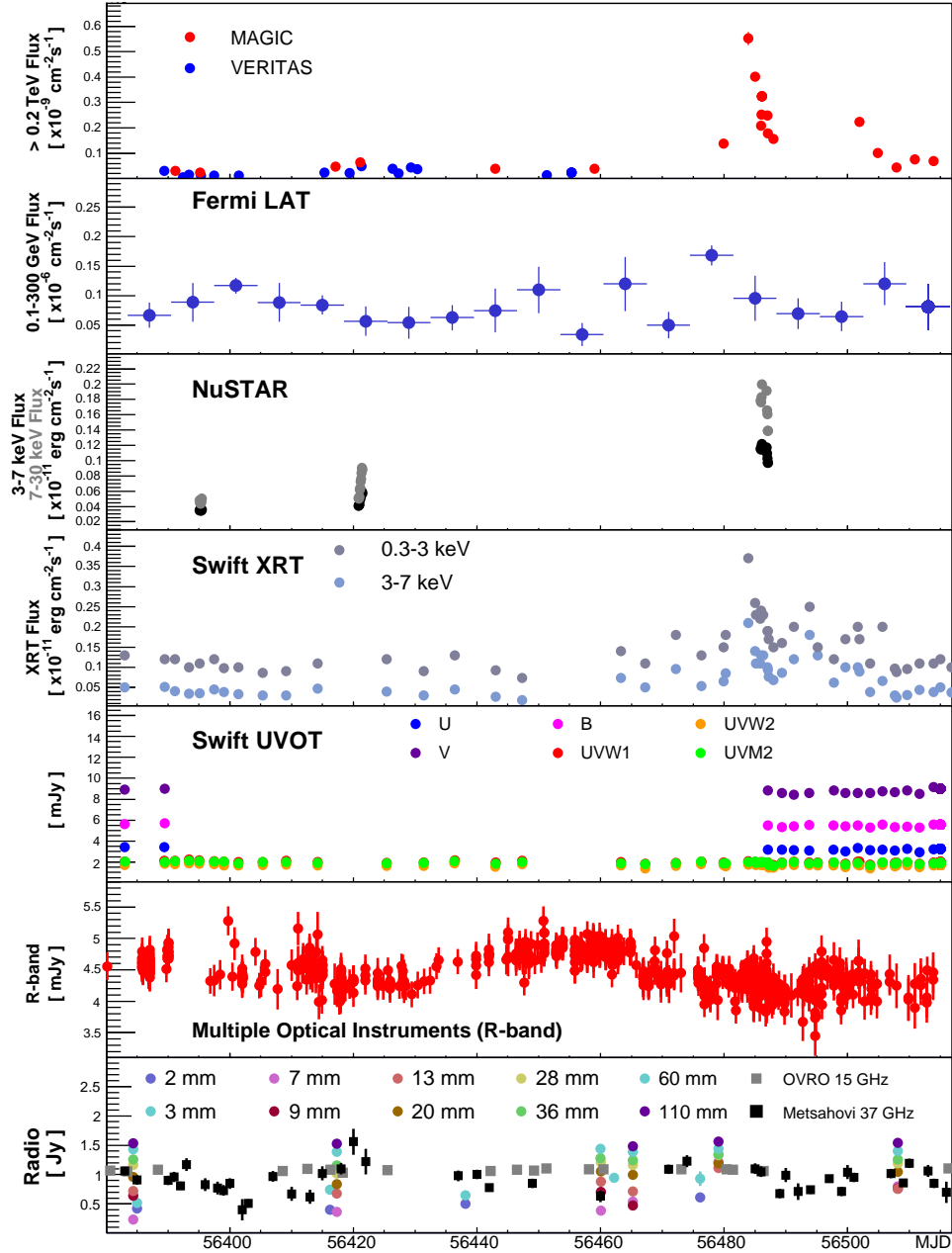
Figure 5. The broadband light curves of Mrk 501 from MJD 56380 to 56520. The VHE data are shown with statistical error bars only. Optical data are corrected as described in Section 3.4. All radio light curve points for 2-110mm are provided by the F-Gamma consortium.
