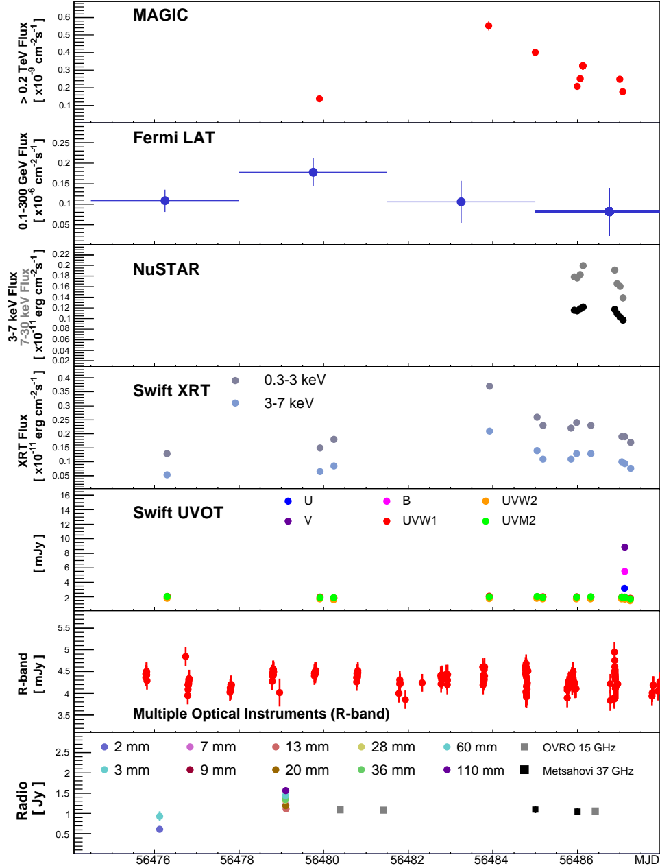
Figure 6. The broadband light curve zoomed in to the period of the elevated X-ray and VHE gamma-ray state.
