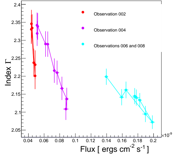
Figure 3. The log-parabolic fit index \Gamma at 10 keV versus the 7-30 keV integral flux for NuSTAR , binned by orbit. The first exposure is shown in red, the second in violet, and the last two in cyan, with solid lines meant to guide the eye along the parameter evolution over the full observations. In all three cases, the spectrum hardens when the intensity increases; in the fourth observation, the spectrum then softens as the intensity decreases.
