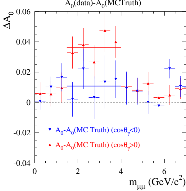
FIG. 18: The difference between the measured asymmetry slope in the \mu^+\mu^-\gamma process and the AfkQed prediction, as a function of m_{\mu\mu} , excluding the J/\psi 3.0-3.2 GeV/ c^2 region. Forward ( \cos\theta_\gamma^* > 0 ) and backward ( \cos\theta_\gamma^* < 0 ) hemispheres are analysed separately. Statistical uncertainties only.
