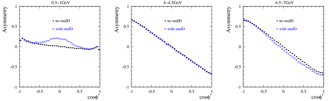
FIG. 12: Raw charge asymmetry as a function of \cos \phi^* in selected m_{\mu\mu} intervals, for e^+e^- \rightarrow \mu^+\mu^-\gamma MC events with ( \circ ) and without ( \bullet ) the two-muon identification, where the events are already required to be within the kinematic acceptance and have two good charged-particle tracks reconstructed.
