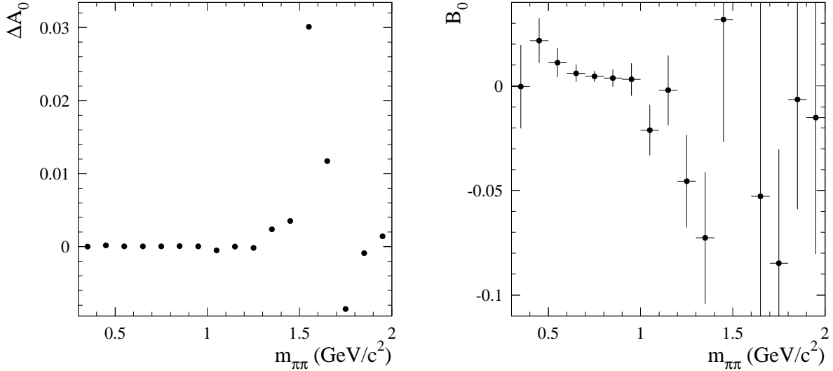
FIG. 25: The change of slope \Delta A_0 (left) and constant term B_0 (right) in the fit of charge asymmetry to A_0 \cos \phi^* + B_0 , as a function of \pi\pi mass for e^+e^- \rightarrow \pi^+\pi^-\gamma .
