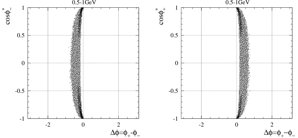
FIG. 13: (left) Distribution of \cos \phi^* vs. \Delta\phi for the N_- sample ( \phi_-^* \in [0, \pi] ) in the (0.5\text{--}1.0)\text{ GeV}/c^2 mass interval for the \mu^+\mu^-\gamma MC; (right) the same for the N_+ sample ( \phi_+^* \in [0, \pi] )
