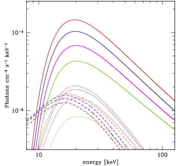
FIG. 15.— Best-fitting model for the main hard X-ray components: the solid lines represent the direct continuum component, the dotted lines represent the forward-scattered component, and the dashed lines represent the back-reflected continuum component. As in Fig. 8, the green, magenta, blue and red lines represent the L, M, H and SH states, respectively.
