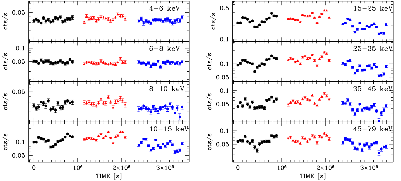
FIG. 4.— Light curves in bins of 5500 s ( \sim 1 satellite orbit). The count rates are the mean values between those detected by the FPMA and FPMB modules, corrected for livetime, PSF losses and vignetting, but not for background. Left panel , from top to bottom: 4 – 6 keV, 6 – 8 keV, 8 – 10 keV and 10 – 15 keV count rates. Right panel , from top to bottom: 15 – 25 keV, 25 – 35 keV, 35 – 45 keV and 45 – 79 keV count rates. Black dots, red triangles and blue squares refer to observations in February, June and July, respectively. The real time interval between black dots and red triangles is about 4 months, whereas between red triangles and blue squares is about 1 month. The y-axis dynamic range is 0.9 in logarithmic scale, in each panel.
