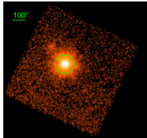
FIG. 2.— 3–79 keV NuSTAR image for the June observation and FPMA module. The image was smoothed with a Gaussian filter with \sigma = 1.5 . The green circle is centered on the peak of the emission and has a radius of 75'' .
