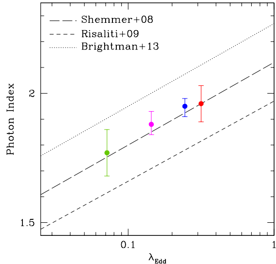
FIG. 16.— Photon index versus the Eddington ratio for the L (green), M (magenta), H (blue) and SH (red) states. The long dashed, short dashed and dotted lines indicate the analytical fit found by Shemmer et al. (2008), Risaliti et al. (2009) and Brightman et al. (2013), respectively.
