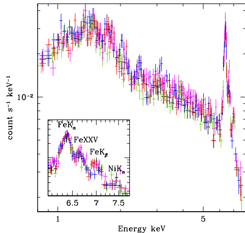
FIG. 9.— Suzaku XIS data in the 0.8 – 8 keV energy range. The colors represent the five observations (see Table 2). The inset panel shows a zoom of the iron complex (i.e. \text{FeK}_{\alpha} , \text{FeK}_{\beta} and Compton shoulder, \text{FeXXV} ) and the nickel emission line.
