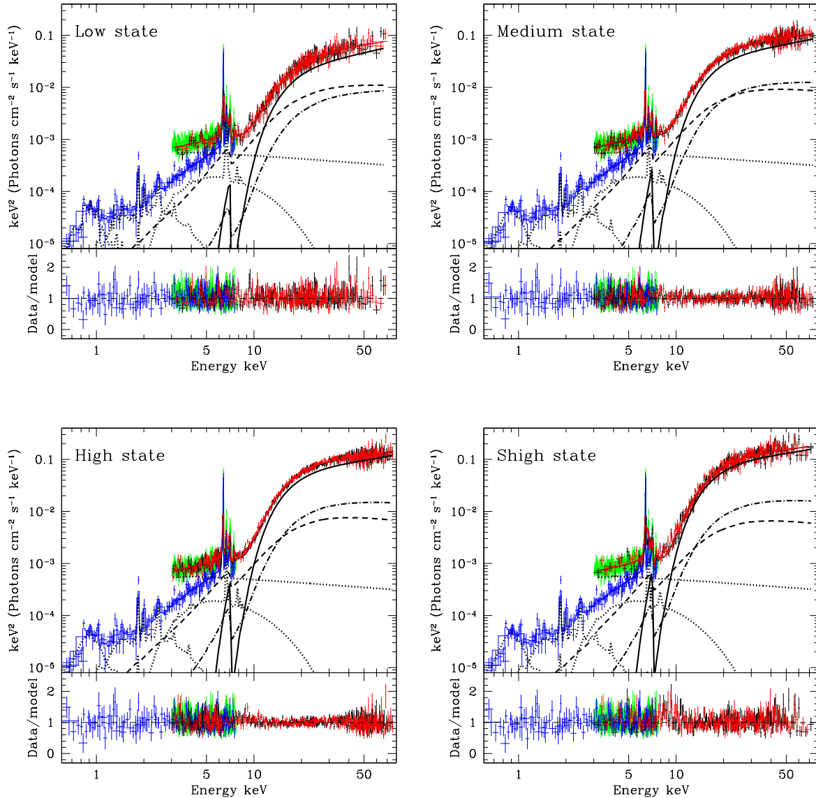
FIG. 12.— The broad-band best-fit spectra, models (upper panels) and residuals (lower panels) for the L, M, H and SH states (from top to bottom, clockwise). The NuSTAR (black is FPMA, red is FPMB), the five Suzaku (green) and Chandra (blue) spectra unfolded with the instrument responses (for single Suzaku and Chandra spectra see Fig. 9 and 11, respectively) are reported in the upper panels. The total model, including the \text{Fe}K_{\alpha} , \text{Fe}K_{\beta} and Nickel lines (not shown as single components for clarity), is superimposed. The model single continuum components are also shown: the primary continuum (black solid lines), the back-reflection (black dashed lines), the forward-reflection (black dashed-dotted lines), the three thermal spectra and the power-law due to the contribution of the serendipitous sources in the NGC4945 field (black dotted lines). In the lower panels the data/best-fit model ratios are shown.
