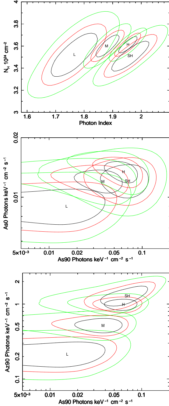
FIG. 13.— 68%, 90% and 99% confidence contours for the L, M, H and SH states for different model parameters. Top panel : column density N_H versus photon index for the direct continuum; middle panel : normalization of the back-reflected continuum versus normalization of the forward-scattered continuum; bottom panel : normalization of the back-reflected continuum versus the normalization of the direct continuum.
