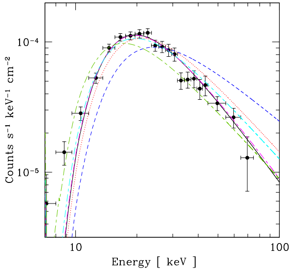
FIG. 10.— The spectrum obtained by subtracting the L state spectrum from the SH state spectrum (black solid points). The lines show the best-fit model allowing variations of: i): normalization of the primary continuum (red dotted line), ii): photon index of the primary continuum (blue short dashed line), iii): absorbing column density of the primary continuum (olive short dashed-long dashed), iv): i)+ii) (black solid line), v) i)+iii) (cyan long-dashed line), vi): i)+ii)+iii) (magenta dotted-short dashed).
