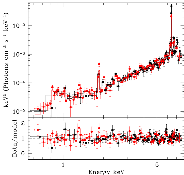
FIG. 11.— The Chandra spectra, unfolded with the instrument response, of the NGC4945 nucleus plus X-ray plume; with the two co-added 2004 observations performed by HETG (zereth) shown in black, and the 2000 observation performed by ACIS-S shown in red (see Table 2). Lower panel shows the data/model residuals.
