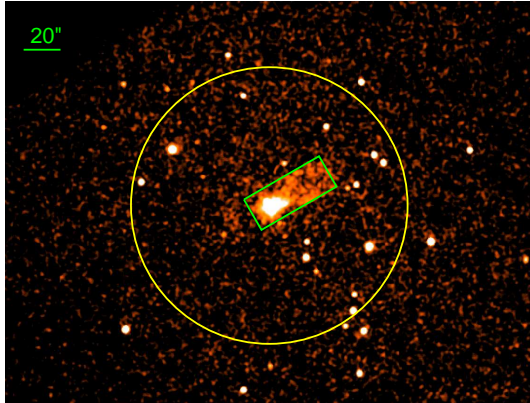
FIG. 3.— 0.5 – 7 keV image mosaic of the three Chandra observations (see Table 2). The green 47'' × 19'' box marks the region used to extract the Chandra spectra, which includes the nuclear source plus a spectrally soft, conically shaped X-ray plume (Schurch et al. 2002, Done et al. 2003). The yellow circle (75'' radius) marks the NuSTAR source extraction region.
