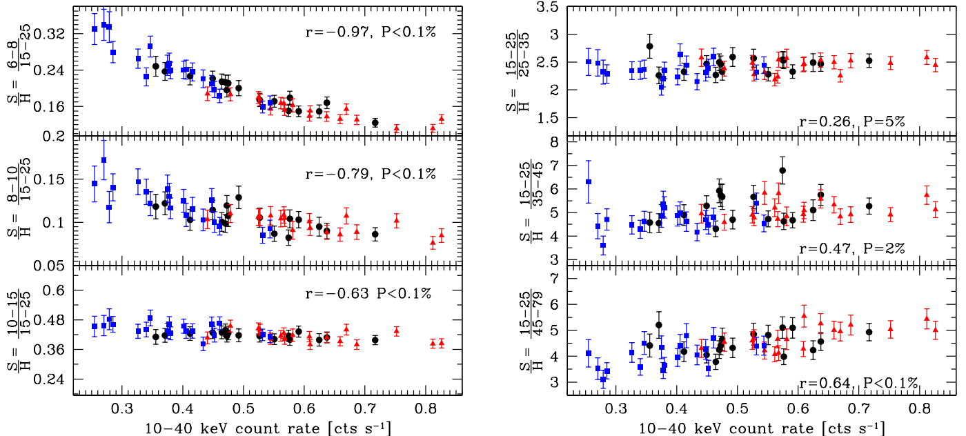
Fig. 5.— Hardness ratio versus count rate in the 10–40 keV range. Black dots, red triangles and blue squares have the same meaning as in Fig. 4. The hardness ratio is evaluated by the relation \frac{S}{H} , where S and H are the count rates in two selected energy ranges, H being harder than S. Left panel: top \frac{6-8}{15-25} ; middle \frac{8-10}{15-25} ; bottom \frac{10-15}{15-25} . Right panel: top \frac{15-25}{25-35} ; middle \frac{15-25}{35-45} ; bottom \frac{15-25}{45-79} . Each panel shows the Spearman rank correlation coefficient r between the total hardness ratio and the count rate in the energy range 10–40 keV; P is the probability that the correlation is not statistically significant, evaluated by the Student's t test.
