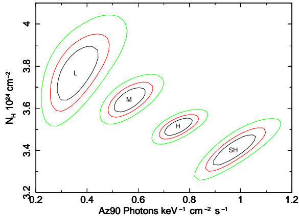
FIG. 14.— 68%, 90% and 99% confidence contours for the column density N_{\text{H}} versus the normalization of the direct continuum, for the L, M, H and SH states. The confidence contours are for the “decoupled” MYTORUS model with the photon index for the direct continuum fixed to 1.9.
