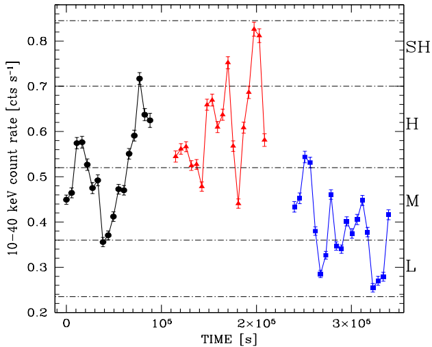
Fig. 6.— Count-rate light curves in the 10–40 keV energy range, in bins of 5500 s ( \sim 1 satellite orbit). The symbols are the same as in Fig. 4. The light curves are divided into four count rate ranges, marked by the dot-dash lines and capital letters on the right (see § 5.1).
