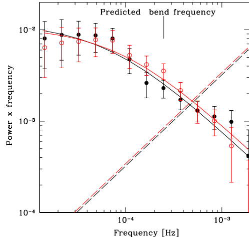
FIG. 7.— Power density spectra in the 10 – 79 keV band for FPMA (black filled circles) and FPMB (red open circles). The error bars represent only the stochastic nature of red-noise light curves. The solid lines represent the best-fitting models for each focal plane module. The dashed lines represent the Poisson noise level for each focal plane module, which has been subtracted from the power density spectra. In the plot the constant Poisson noise appears as a linearly increasing function and the -1 slope of the low-frequency power spectrum appears horizontal.
