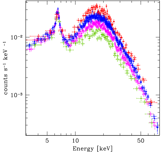
FIG. 8.— NuSTAR spectra in the 3 – 79 keV energy range. The solid dots are FPMA data, open dots are FPMB data. The colors represent: green – L state, magenta – M state, blue – H state and red – SH state.
