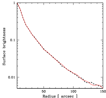
FIG. 1.— 3–79 keV source brightness profiles for the July observation. The red solid profile is the result obtained using the cleaned event file produced with the standard analysis; the black dashed profile is the result of the non-standard analysis.
