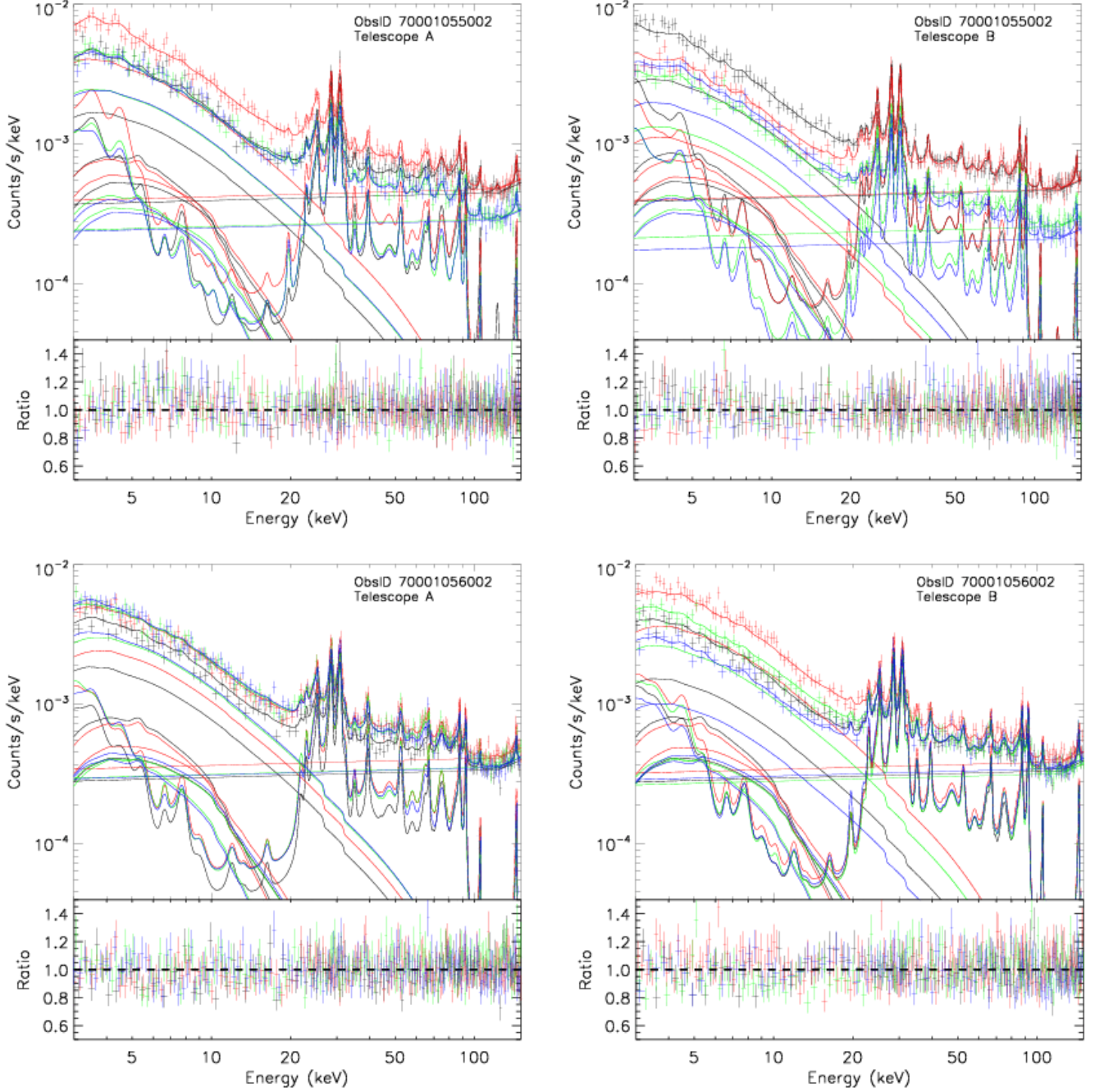
FIG. 14.— Simultaneous fit of the model background to the 16 spectra extracted from the regions shown in Figure 13, with the spectra in each panel associated with a single observation and focal plane as labeled; the black, red, green, and blue data (crosses) and model components (lines) correspond to regions 1, 2, 3, and 4, respectively, as labeled in Figure 13. We fit the two epochs together primarily so that the “Aperture” component can be described by only one free parameter, consistent with the nature of its origin.
