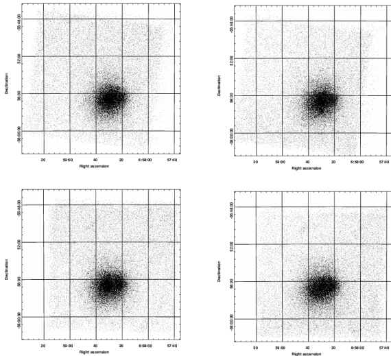
FIG. 1.— Cleaned events projected in sky coordinates from 3–20 keV; pixels with no events are displayed white while pixels with 1 or \geq 2 events are displayed grey or black, respectively. Top row: ObsID 700055002 images; Bottom Row: ObsID 700056002 images. The left and right columns show the data from the A and B telescopes, respectively.
