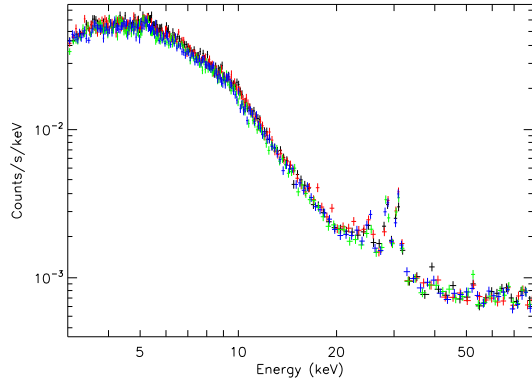
FIG. 3.— Raw spectra from the region indicated in the top left panel of Figure 2, grouped into 15\sigma bins for clarity. ObsID 700055002 spectra are in black (telescope A) and red (B) and ObsID 700056002 spectra are in green (A) and blue (B). Above \sim 20 keV the background dominates each spectrum, causing a flattening and the appearance of lines due to instrumental fluorescence and activation from SAA passages.
