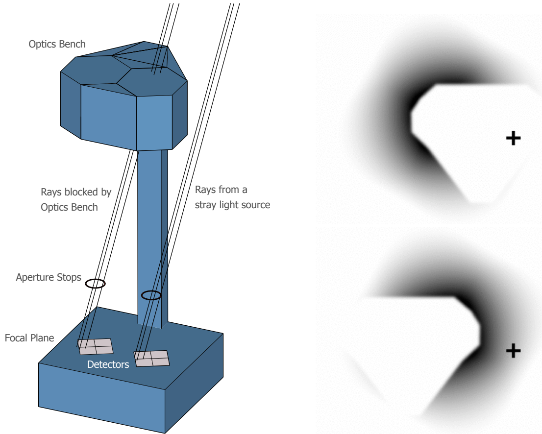
FIG. 8.— Left: A schematic of the observatory that illustrates how far off-axis sources can directly shine on the detectors through the aperture stop, producing the “Aperture” background. In this example, rays from the source are shielded from striking the left detector plane by the optics bench, but other rays from the same source have an unimpeded path through the aperture stop to shine on a corner of the right detector plane. Right: The location of sources on the sky, as visible from the detector plane, that produce the “Aperture” background for Telescopes A (top) and B (bottom). The images are weighted (darker) by the number of detector pixels a given source shines on. The crosses give the approximate position of the source shown in the left panel.
