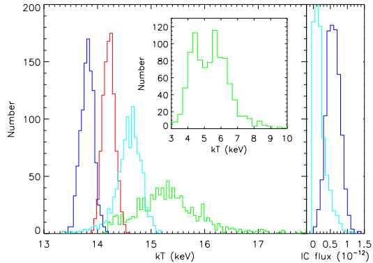
FIG. 6.— Best-fit temperatures from the 1T (red), 2T (green), T+IC (fixed \Gamma = 1.86 , blue), and T+IC (free \Gamma , cyan) models fit to the Bullet cluster spectrum using 1000 realizations of the background that include systematic fluctuations. The background minimally affects the temperature components that depend primarily on high signal-to-noise parts of the spectrum, as in the 1T and T+IC cases, but has a much stronger impact on the 2T components ( kT_{\text{low}} shown in inset panel while kT_{\text{high}} shown in the main panel) which are more sensitive to lower signal-to-noise bins. The right panel shows the distribution of the best-fit power law fluxes (50–100 keV, units of ergs s^{-1} cm^2 ) for the IC components.
