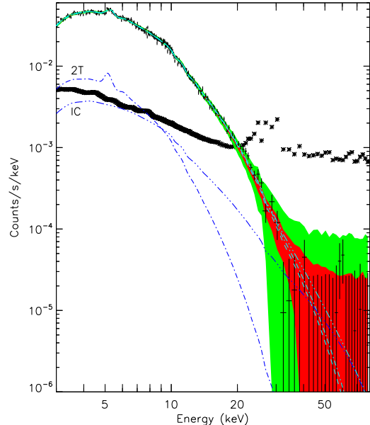
FIG. 4.— The background-subtracted Bullet cluster spectrum (crosses, using the nominal background model; all spectra from Figure 3 have been combined for clarity) shown together with the background (“*” symbols) and the 1\sigma (red/dark shaded region) and 3\sigma (green/light shaded region) effect of background uncertainties relative to the 1T model. The shaded regions indicate the range within which the spectrum might shift due to statistical and systematic fluctuations in the background relative to our nominal background model. The components for the three best-fit models are shown in blue for the 1T, 2T, and T+IC (with \Gamma fixed at 1.86) cases with the dashed, dot-dashed, and dot-dot-dot-dashed lines, respectively. The less dominant component for the 2T and T+IC models are labeled and show the lower temperature component and IC component, respectively.
