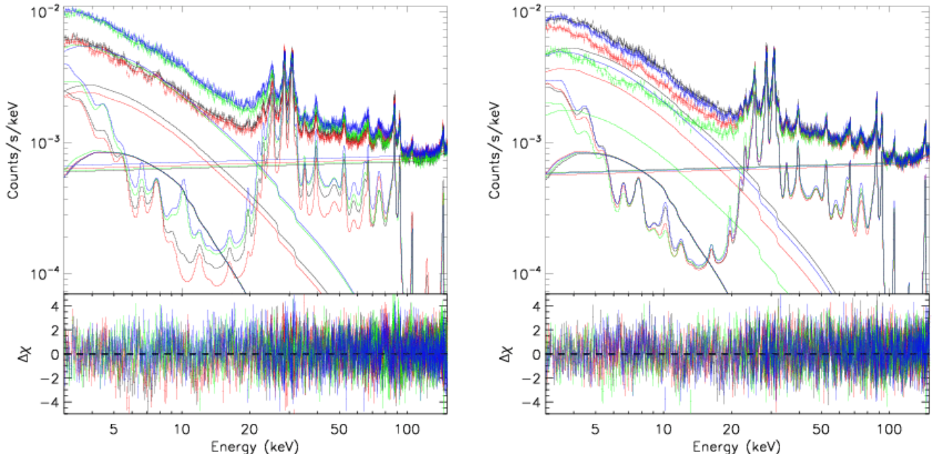
FIG. 12.— The background model fit to the blank sky spectra from focal planes A (left panel) and B (right panel), separated by detector: Det0 (black), Det1 (red), Det2 (green), and Det3 (blue). The spectral shapes of each component are fixed, but the normalizations are free to vary to account for differences between detectors.
