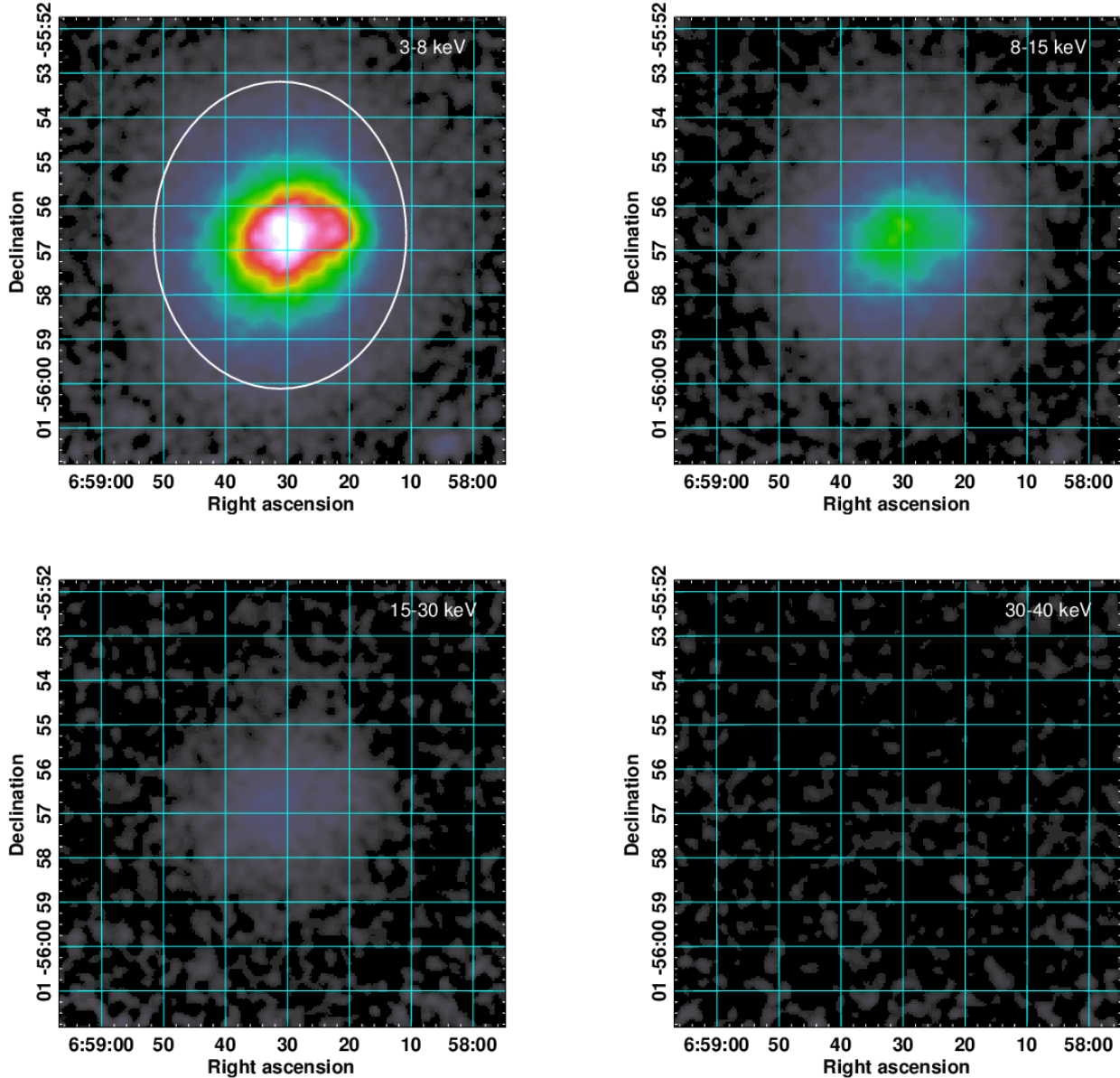
FIG. 2.— Background-subtracted and exposure-corrected images combined from both observations and telescopes. Images are presented on a linear scale from 0 counts/s/pix (black) to 5 \times 10^{-5} counts/s/pix (white). The energy band of each image is shown clockwise from top left: 3–8 keV, 8–15 keV, 30–40 keV, and 15–30 keV. The ellipse in the top left panel indicates the region from which spectra are extracted. Images are smoothed with a uniform Gaussian kernel of \sigma = 12.3'' (5 pixels). Although fewer cluster counts are detected at higher energies, no obvious change in morphology occurs relative to the 3–8 keV image, which is dominated by thermal photons.
