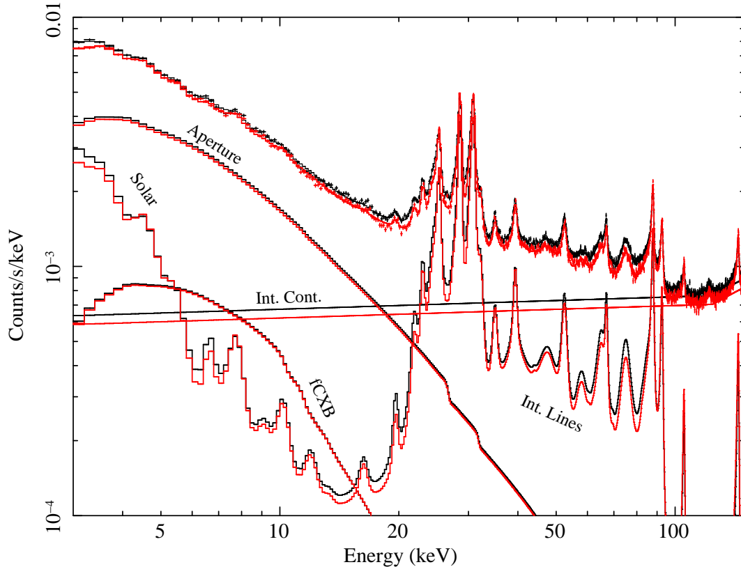
FIG. 9.— Initial independent fits to stacked blank sky data for telescopes A (black) and B (grey or red). The spectra for each of the four detectors in each focal plane are averaged together when combined, such that the rates shown are also per detector. The major contributions are labeled according to their source with the “Aperture,” “fCXB,” and “Solar” components having a cosmic origin and the “Int. Cont.” and “Int. Lines” having an “internal” or instrumental origin, due largely to the spacecraft environment. Because the spectral shapes are identical, the “Aperture” component consists of both emission directly from the CXB through the aperture stop and from CXB emission reflected/scattered off the backside of the aperture stop and/or other parts of the telescope.
