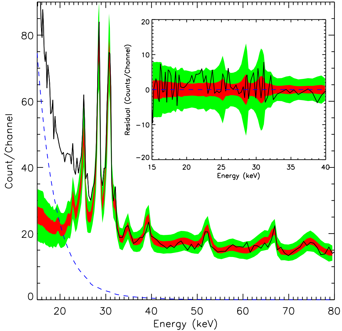
FIG. 15.— The Bullet cluster spectrum at hard energies (solid line) is shown with the 1\sigma (red; dark gray) and 3\sigma (green; light gray) ranges given by the 1000 background realizations. The dashed (blue) line indicates the average 1T thermal model contribution to the spectrum. The inset plot gives the residual of the fit to the thermal model after background subtraction, with the same shaded regions displayed in the main plot illustrating the extent of fluctuations expected from the background alone. While the nominal background model appears too low just above 20 keV and too high from \sim 35 –55 keV, it is clear these variations are not extreme.
