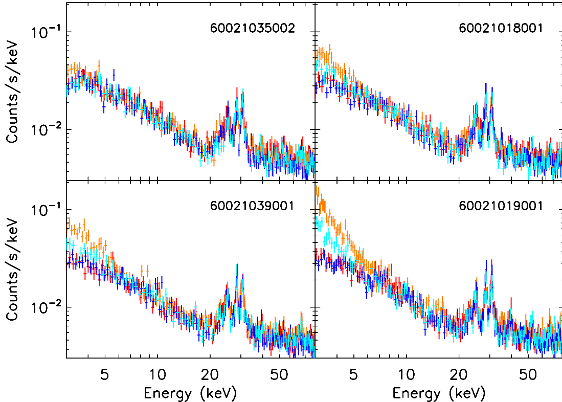
FIG. 11.— Four observations of COSMOS fields, with the data from each telescope separated into periods when the spacecraft is in the Earth’s shadow (A: red, B: blue) and when it is illuminated by the Sun (A: orange, B: cyan). These spectra show how fluctuations in solar activity can increase the low energy background, and that more reflected solar emission is apparently visible to A.
