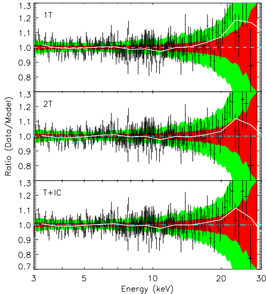
FIG. 5.— The ratio of the spectrum (crosses, using the nominal background model; all spectra from Figure 3 have been combined for clarity) to each model. The red/dark and green/light shaded regions are the same as in Figure 4. Although difficult to tell, the 2T and T+IC models better describe the overall spectral shape from 3–20 keV, producing flatter residuals than the 1T model; the white line in each plot represents the same data shown as crosses but more heavily binned to accentuate the broader spectral shape relative to the models. The rise from 20–22 keV is likely a background line(s) imperfectly subtracted; note that the feature is within our estimated 3\sigma uncertainty for the background reconstruction.
