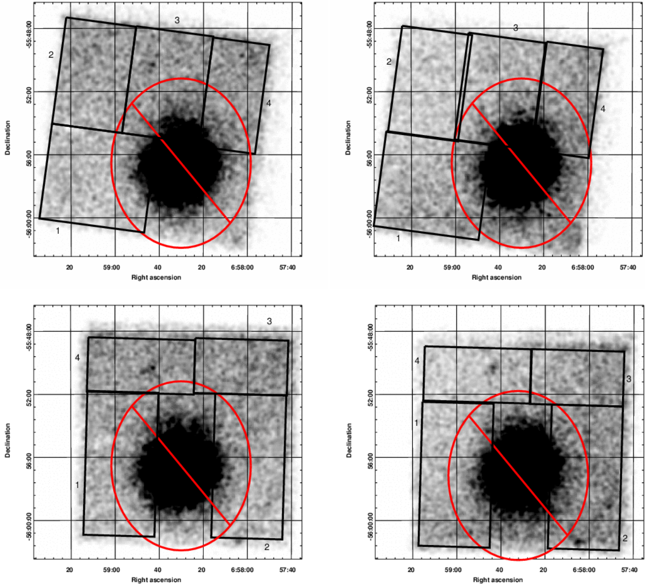
FIG. 13.— The regions from which spectra are extracted to characterize the background; events inside the ellipse are excluded. Data from telescopes A and B are shown in the left and right panels, and the first and second epochs are shown in the top and bottom panels, respectively. The data are the same as in Figure 1: the images have been smoothed by Gaussian kernel of width 5 pixels and scaled between 0 (white) and 1 (black) counts to bring out structure in the background.
