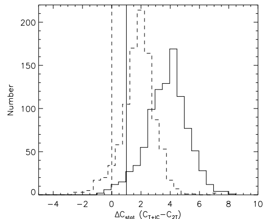
FIG. 7.— The difference of Cash statistic values between the T+IC and 2T models for each of the 1000 background realizations, which include statistical and systematic fluctuations. The solid and dashed histogram and lines refer to fits where the IC components used a fixed ( \Gamma = 1.86 ) or free ( \Gamma \sim 2.4 ) photon index, respectively. Values to the left of the solid/dashed line show realizations in which the T+IC model is favored, while values to the right have the 2T model favored. The solid line is drawn at \Delta C = 1 since the 2T model has one more free parameter than the T+IC model when \Gamma is fixed. For the majority of background realizations, the 2T model is clearly favored over a spectral model including a non-thermal component.
