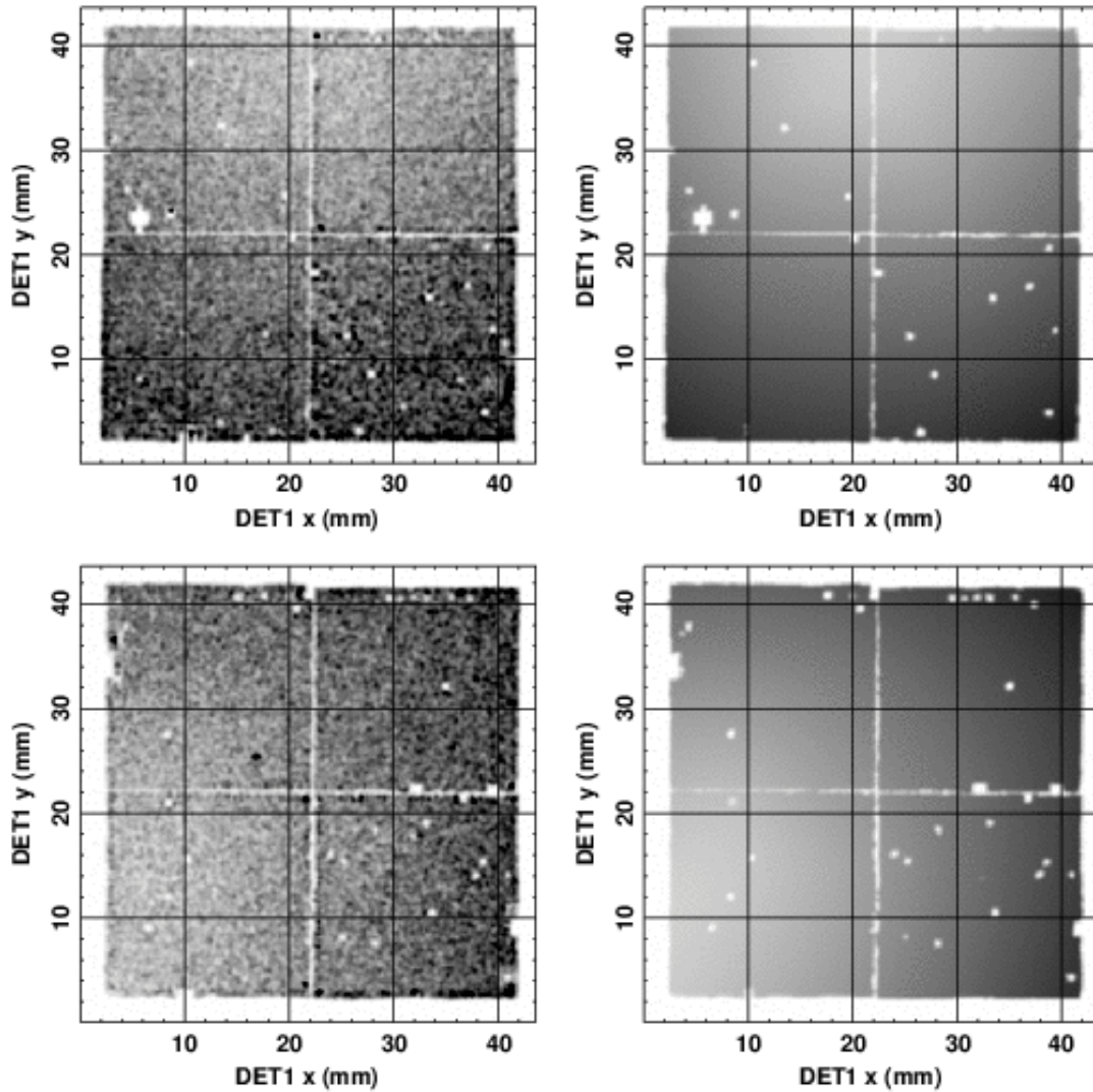
FIG. 10.— Stacked images in the 7–15 keV band for the blank sky fields (left panels) compared to the best-fit model of the spatial distribution of the “Aperture” background (right panels) for telescopes A (top panels) and B (bottom panels). The data include other background components not included in the model, although they are subdominant in this energy band. Excluded RAW (native) pixels display as white, and detectors 0–3 are arranged counterclockwise with detector 0 in the top right of the focal planes. The gradient spans a linear scale from 0 to 4 counts, and the data have been smoothed by a Gaussian kernel of width 3 pixels for clarity.
