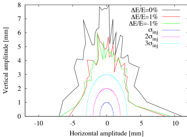
Figure 3: Dynamic aperture.
