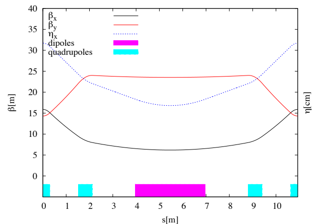
Figure 1: Arc cell.
