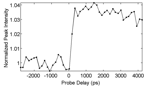
Figure 5: Diffracted intensity as a function of pump-probe time delay at Q=1.535\text{\AA}^{-1} .
