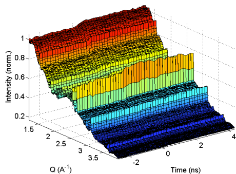
Figure 4: Powder diffraction pattern (Intensity vs. Q(\text{\AA}^{-1}) ) at multiple pump-probe time delays.
