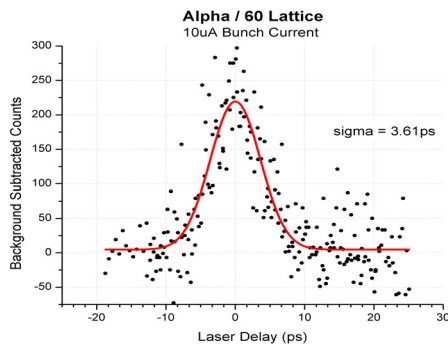
Figure 2: 3.6ps rms cross-correlation measurement in low- \alpha mode with 10uA single bunch current.
