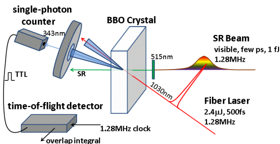
Figure 1: Cross-correlation with sum-frequency geometry.
