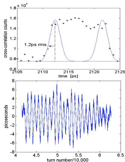
Figure 3: a) 1ps regime cross-correlation measurements taken with b) large phase oscillations.
