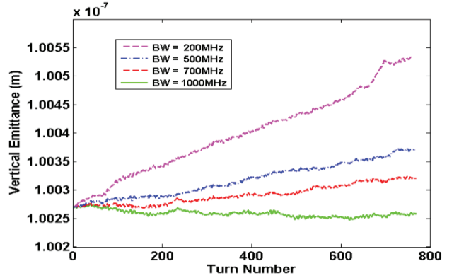
Figure 5: Vertical emittance stabilization with different feedback kicker bandwidth and fixed amplifier gain 0.5.
