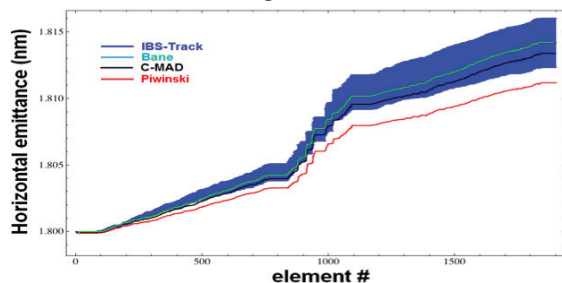
Figure 7: Emittance growth with IBS during one turn in SuperB. C-MAD (black) and IBS-Track (blue) codes, and theoretical models Bane (green) and Piwinski (red).
