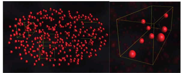
Figure 1: Modelling of IBS. Longitudinal bunch slices are assigned to each computer processor. In each 3D cell (right), Monte-Carlo method is applied in a stochastic process in which beam particles are randomly coupled and the momentum exchanged.
