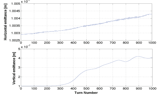
Figure 4: Simulated emittance growth (note vertical > 400%) in the CERN SPS with cloud density 0.5 \times 12e/m^3 and without feedback.
