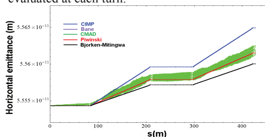
Figure 6: CLIC DR, effect of IBS on the one turn evolution of the horizontal emittance growth. Multi-particle code C-MAD compared with theoretical models.
