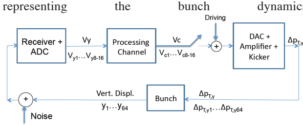
Figure 2: Block diagram of single-bunch feedback system
