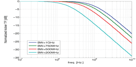
Figure 3: Normalized kicker transfer functions.
