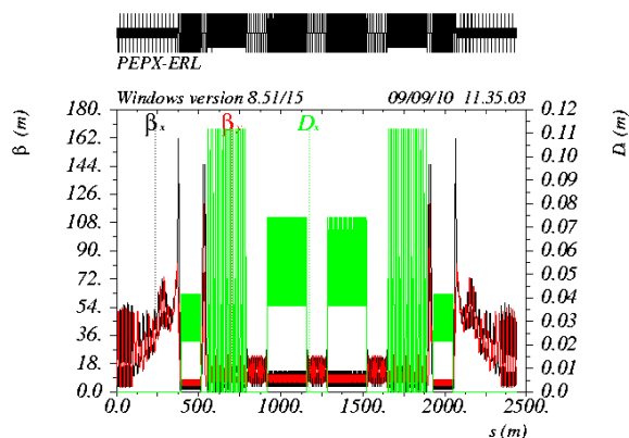
Figure 1: The optics functions of the PEP-X ERL, one recirculation.
