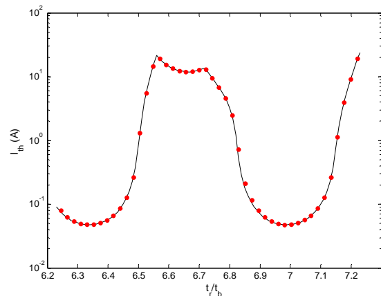
Figure 3: Threshold current obtained by tracking simulation (red dots) and numerical solution (black line) of the dispersion relation Eq. (1).
