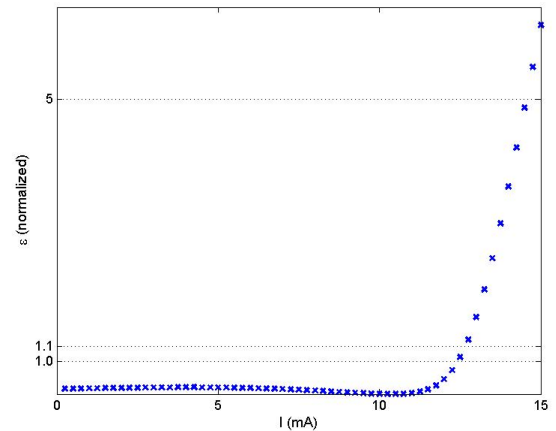
Figure 4: Variation of projected emittance with respect to the beam current.
