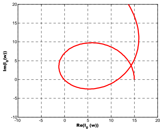
Figure 2: Complex plain of I_0(w) with respect to w obtained from the dispersion relation Eq. (1) for one specific case, n_r = 7 , \delta = 0.27 . The threshold current is obtained to be 11.5 A.
