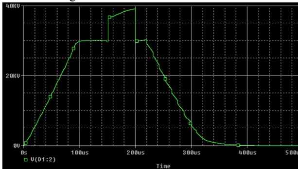
Figure 6. Typical circuit simulation result for the output voltage of the F1 Marx.
