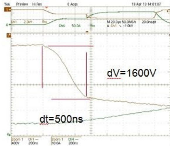
Figure 8. Single "vernier" cell turn-on voltage. Measured dv/dt is 3.2 \text{ kV}/\mu\text{s} .
