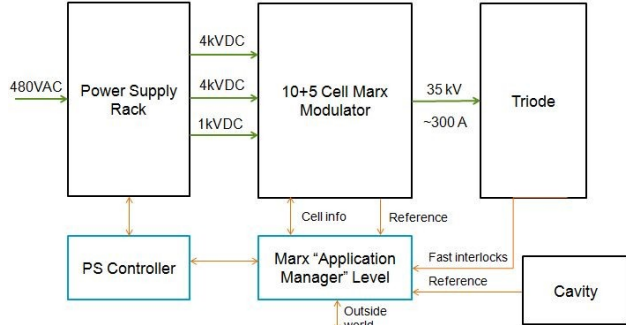
Figure 2. System diagram for the F1 Marx modulator.
