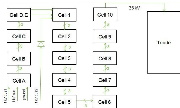
Figure 3. Modulator block diagram for the F1 modulator. The "vernier" cells are denoted by letters (A-E) and the "main" cells are denoted by numbers (1-10).
