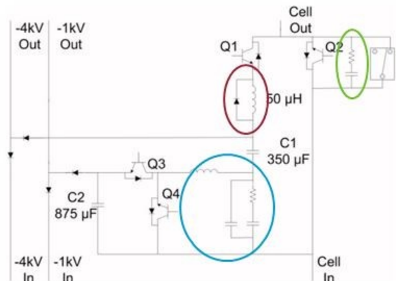
Figure 4. Simple schematic for one SLAC P2 Marx cell. This cell is slightly altered for the F1 Marx by adjusting the PWM filter (blue circle) and the two snubbers (green and brown circles)
