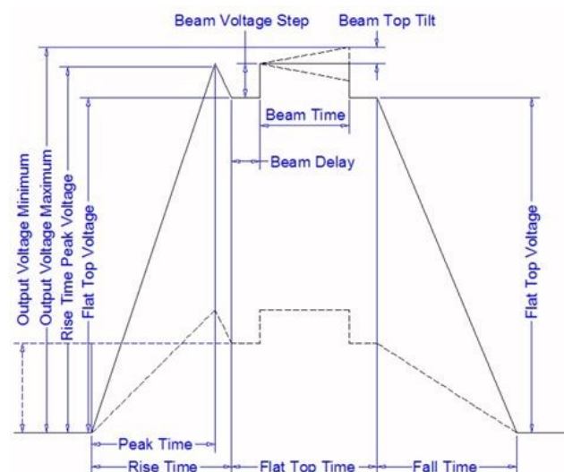
Figure 1. Desired waveform shape for the FNAL triode modulator.
