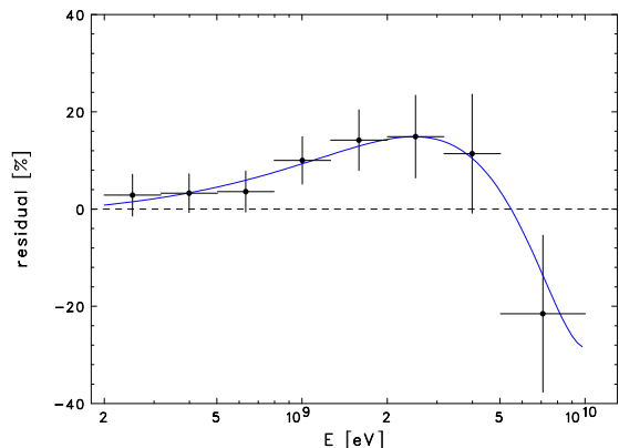
FIG. 4.— The fractional residuals at 8 energy bins in 0.2 to 10 GeV between the observed LAT data and the best-fit Galactic diffuse emission model in the nearby circle centered at (\alpha, \delta)=(288.^\circ 4, 10.^\circ 2) with radius of 0.^\circ 5 . The fluxes of all sources included in the fit-model except for the Galactic diffuse component are subtracted from the observed data. The blue line shows a cubic function fitted to the residual data.
