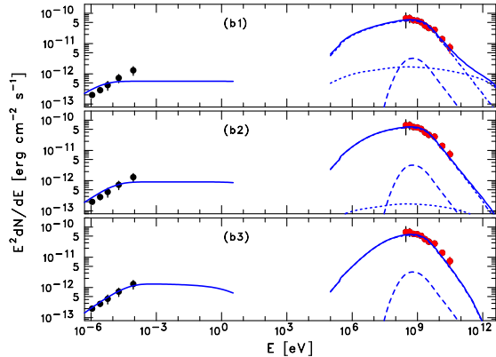
FIG. 10.— Same as Fig. 9 but the gamma-ray emission is assumed to be dominated by electron bremsstrahlung. Cases b1, b2 and b3 represent n_H = 10, 100, 1000 cm^{-3} , respectively (see Table 1).
