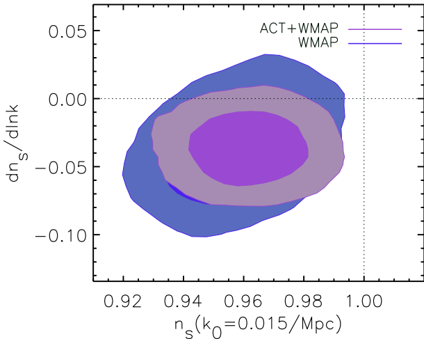
FIG. 7.— Two-dimensional marginalized limits (68% and 95%) for the spectral index, n_s , plotted at the pivot point k_0 = 0.015/\text{Mpc} , and the running of the index dn_s/d\ln k , for ACT+WMAP, compared to WMAP. This model has no tensor fluctuations. A negative running is preferred, but the data are consistent with a power-law spectral index, with dn_s/d\ln k = 0 .
