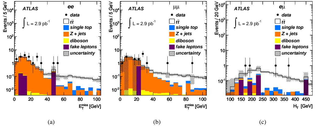
Figure 4: The E_T^{\text{miss}} distribution in the signal region for (a) the ee channel without the E_T^{\text{miss}} > 40 \text{ GeV} requirement, (b) the \mu\mu channel without the E_T^{\text{miss}} > 30 \text{ GeV} requirement, and (c) the distribution of the H_T , defined as the scalar sum of the transverse energies of the two leptons and all selected jets, in the signal region without the H_T > 150 \text{ GeV} requirement.
