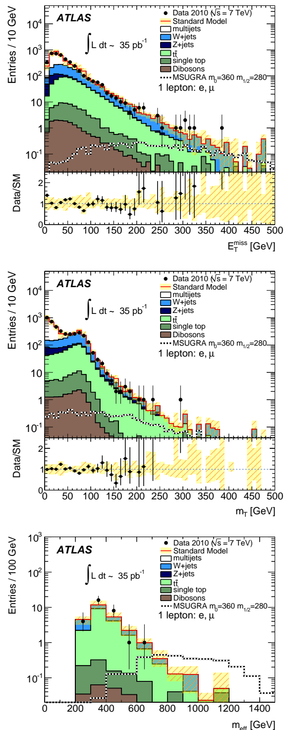
FIG. 1: Top: E_T^{\text{miss}} distribution after lepton and jet selection. Center: m_T distribution after lepton and jet selection. Bottom: Effective mass distribution after final selection criteria except for the cut on the effective mass itself. All plots are made for the electron and muon channel combined. Yellow bands indicate the uncertainty on the Monte Carlo prediction from finite Monte Carlo statistics and from the jet energy scale uncertainty.
