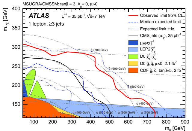
FIG. 2: Observed and expected 95% CL exclusion limits, as well as the \pm 1\sigma variation on the expected limit, in the combined electron and muon channels. Also shown are the published limits from CMS [3], CDF [4], and D0 [5, 6], and the results from the LEP experiments [29].
