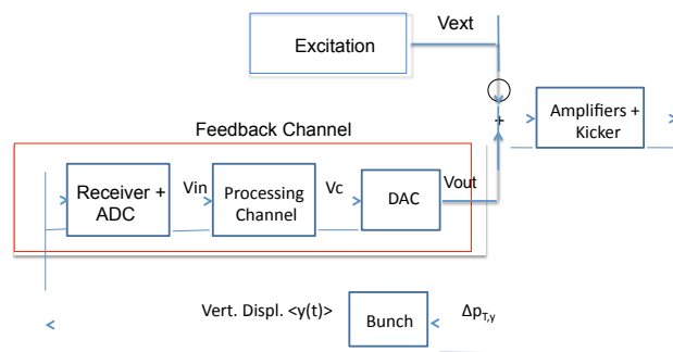
Figure 1: Loop topology for measuring beam dynamics changes due to feedback. An excitation signal V_{\text{ext}} drives the beam, while the closed loop feedback acts in response to the excitation. Time-domain samples of the excitation, and the beam response V_{\text{in}} are processed in both time and frequency domains.
