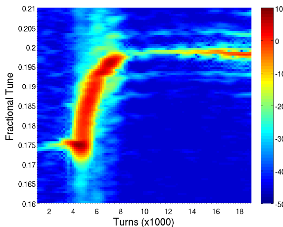
Figure 4: Frequency-domain spectrogram of unstable (no feedback) beam motion with charge loss. The machine chromaticity is ramped to zero at 2000 turns, resulting in mode zero unstable beam. The dramatic tune shift is a sign of charge loss due to the unstable motion.
