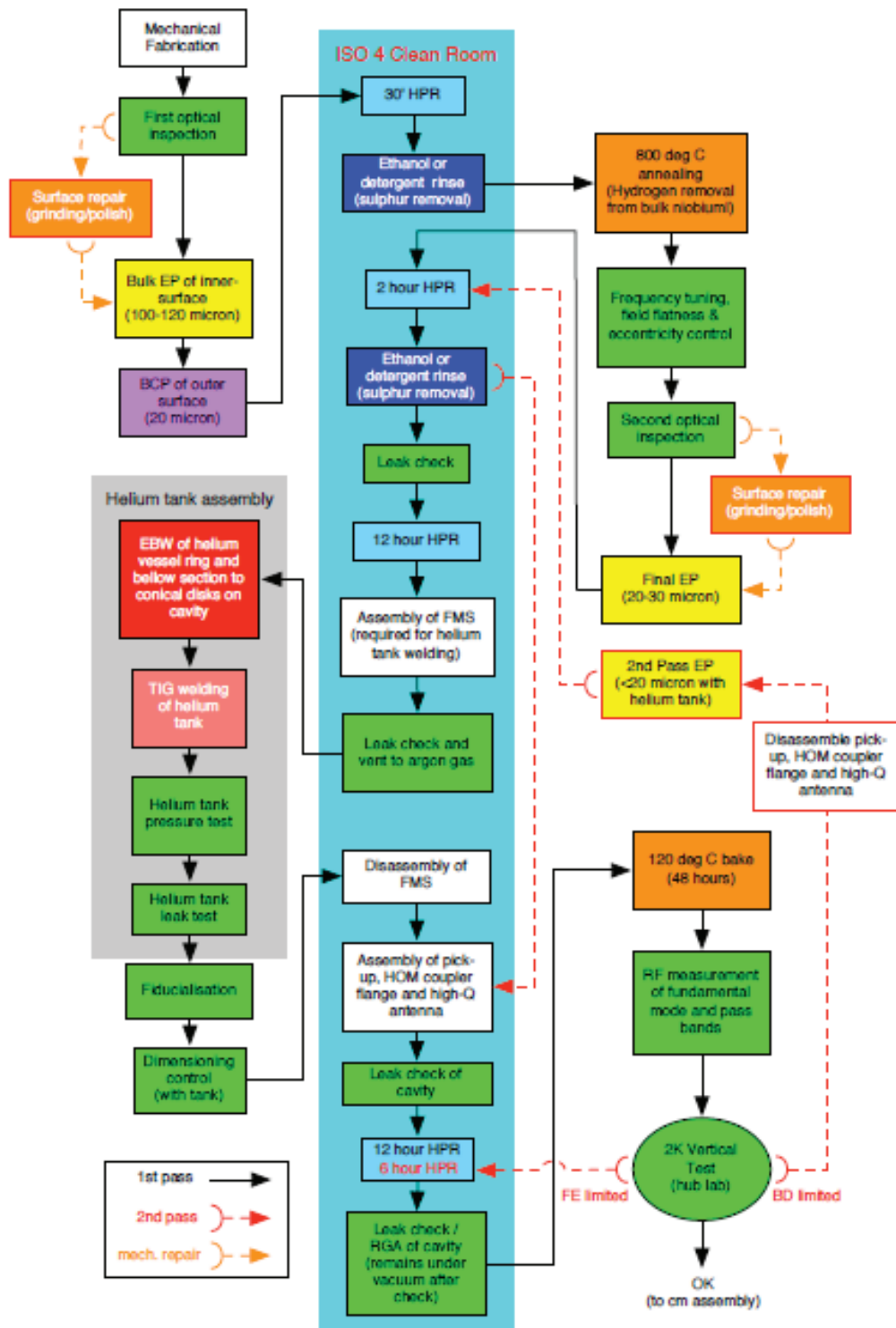
Figure 1: Cavity Processing and testing steps as adopted for the European XFEL [18].
